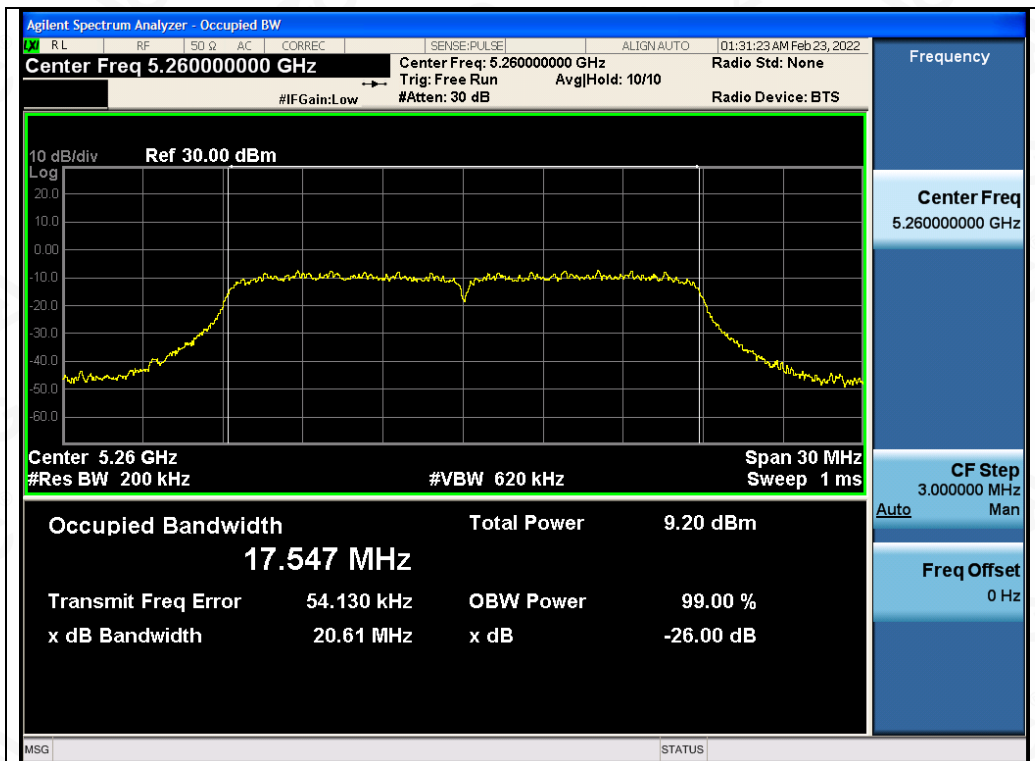
Test_Graph_802.11ac20_ANT2_5260_MCS0_OBW
