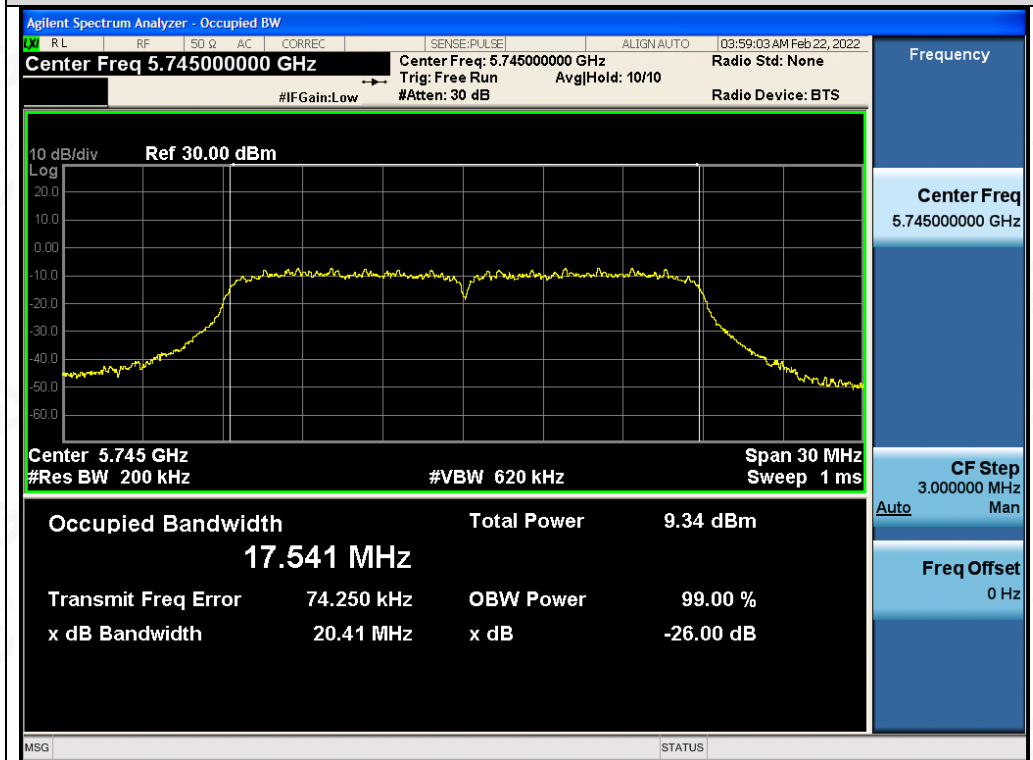
Test_Graph_802.11n20_ANT1_5745_MCS0_OBW
