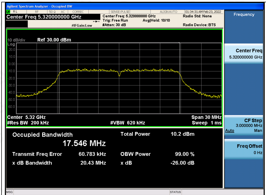
Test_Graph_802.11ac20_ANT2_5320_MCS9_OBW
