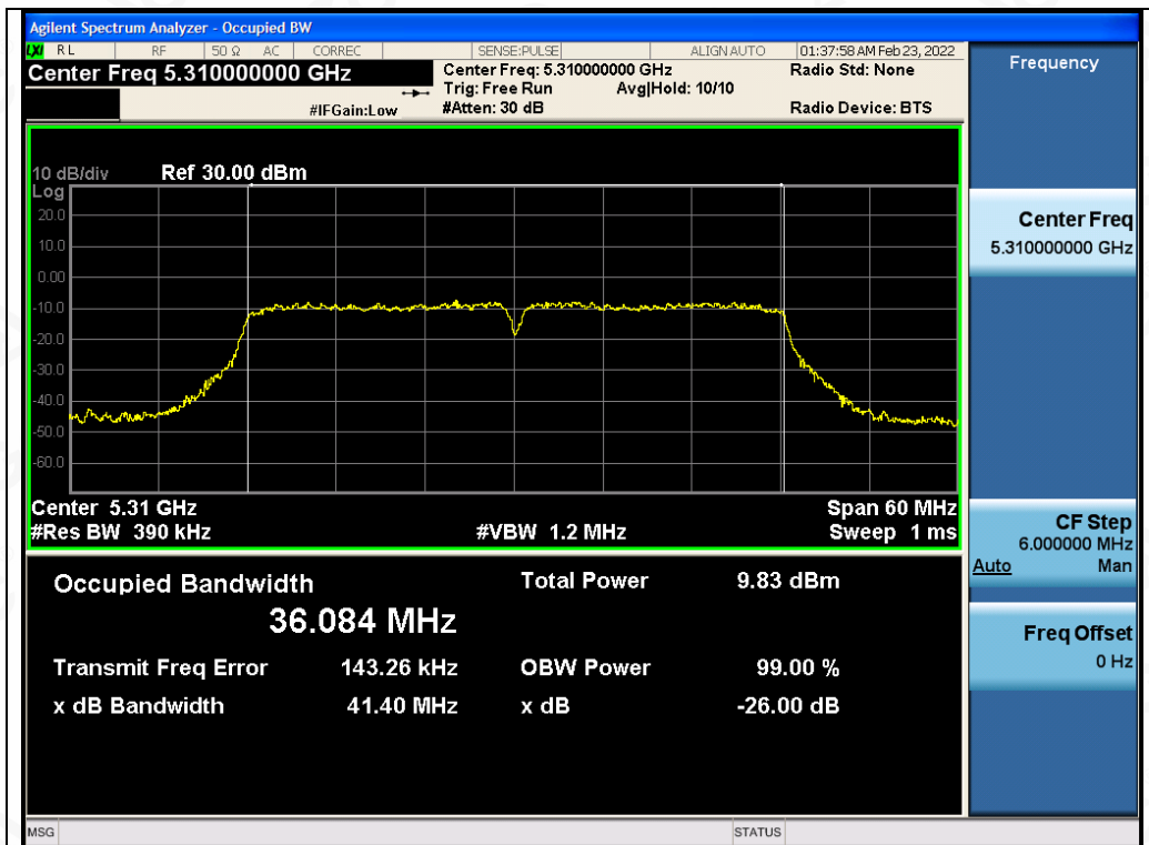
Test_Graph_802.11ac40_ANT2_5310_MCS9_OBW
