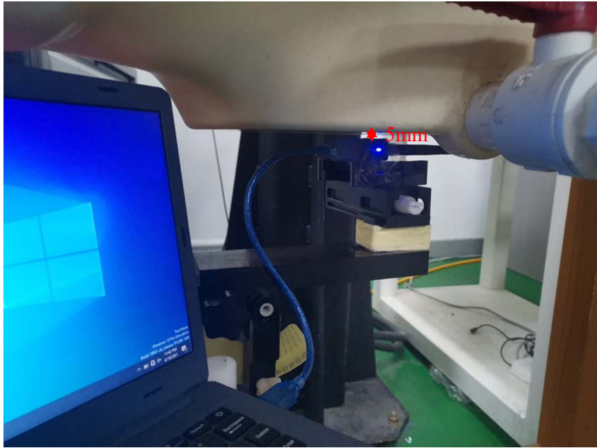
Vertical-Front Setup Photo (5mm)
