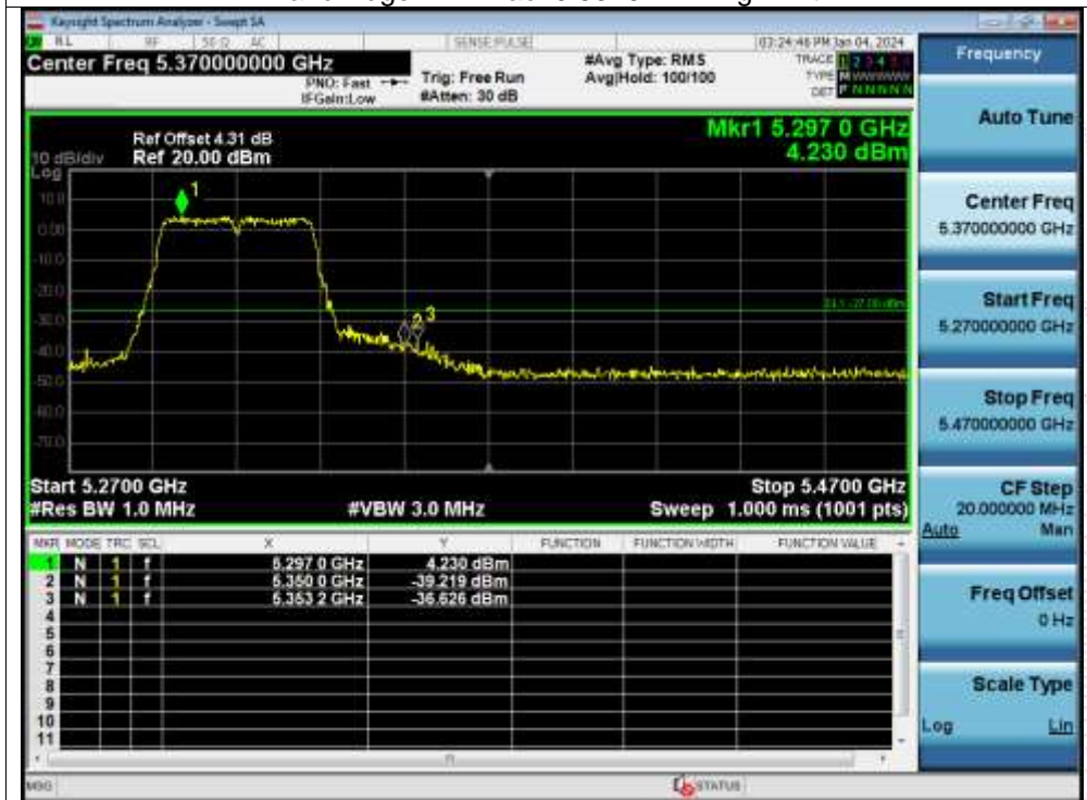
Band Edge NVNT ac40 5310MHz High Ant1
