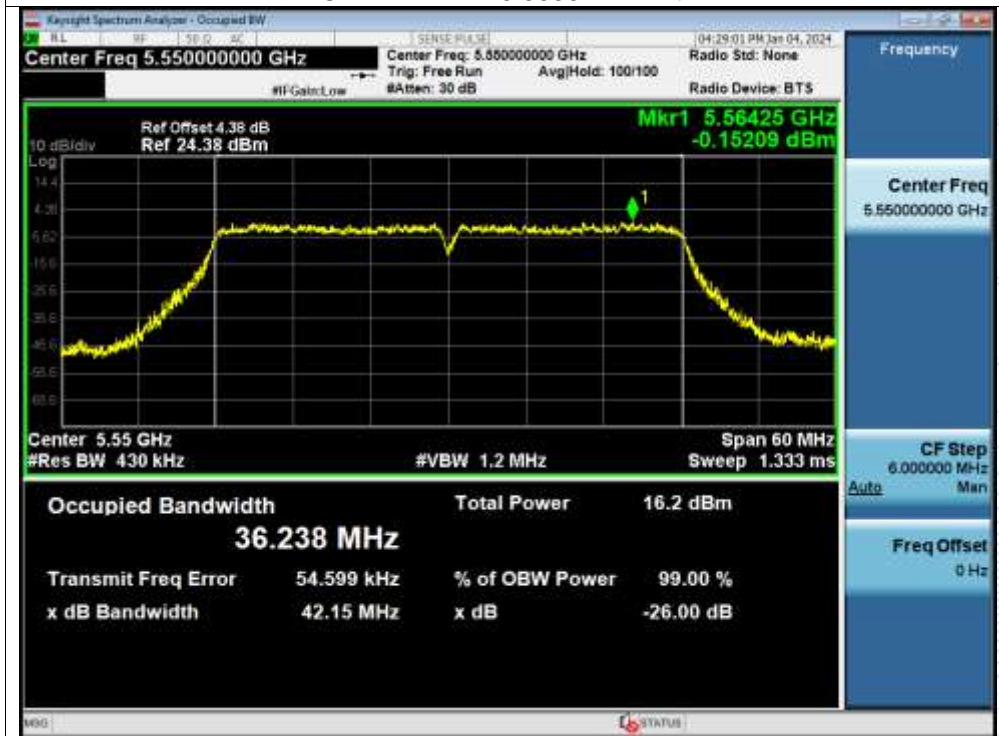
OBW NVNT n40 5550MHz Ant1
