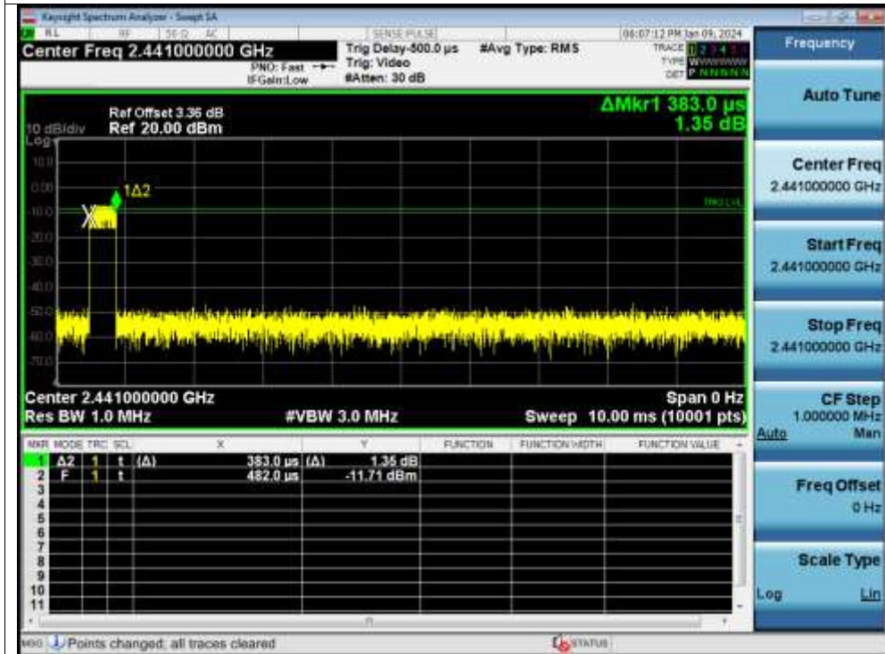
Dwell NVNT 1-DH1 2441MHz Accumulated
