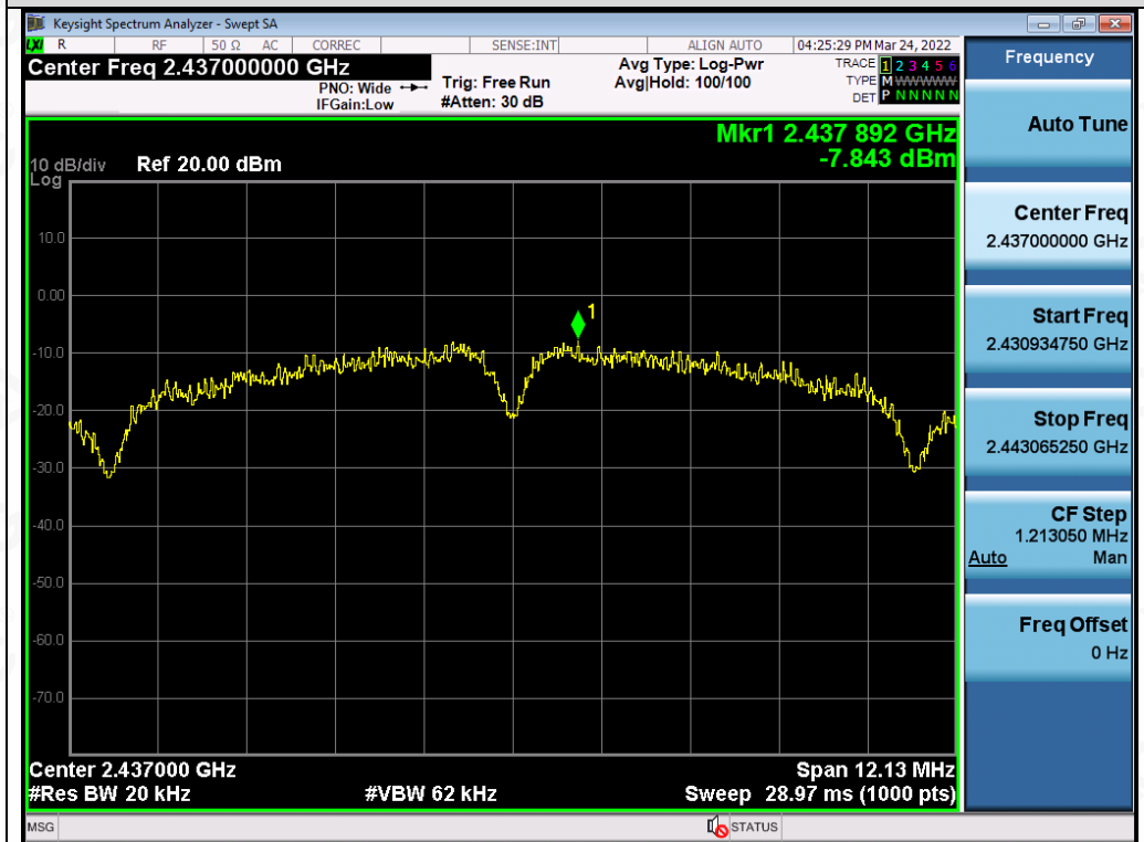
Test_Graph_802.11b_ANT2_2437_1Mbps_PSD
