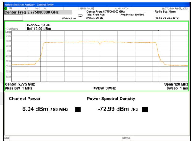
5775MHz_AV_Ant B
