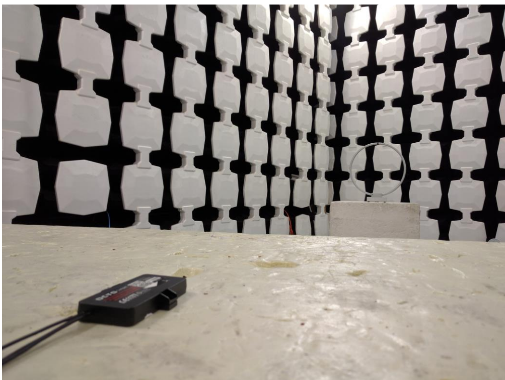
Radiated Spurious Measurement(Blow 30MHz) Setup
