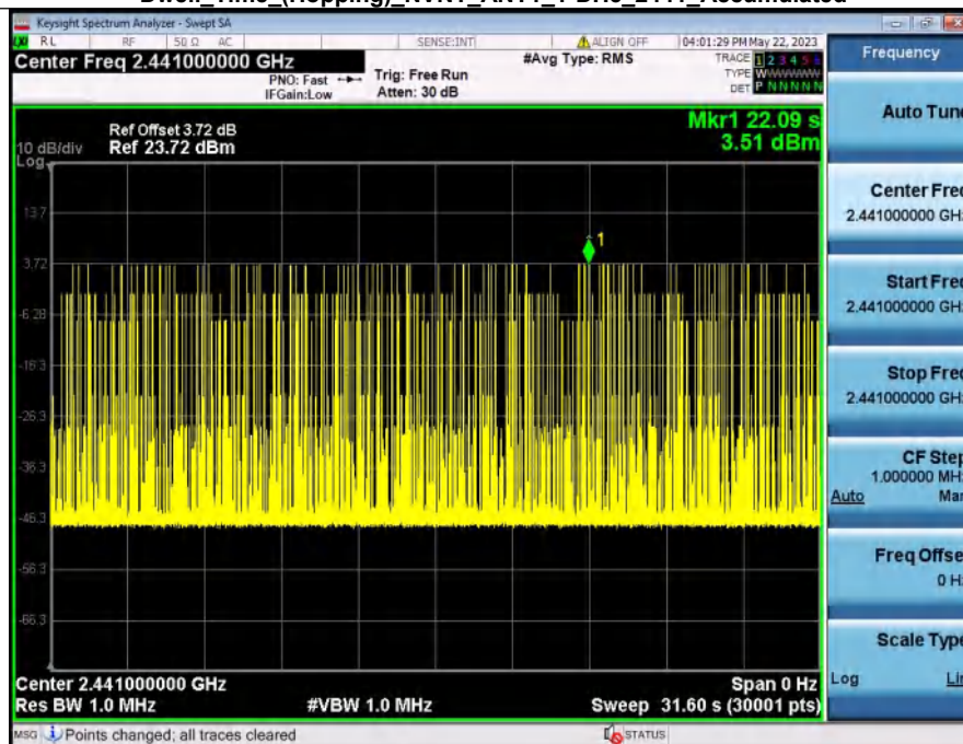
Dwell_Time_(Hopping)_NVNT_ANT1_1-DH5_2441_Accumulated
