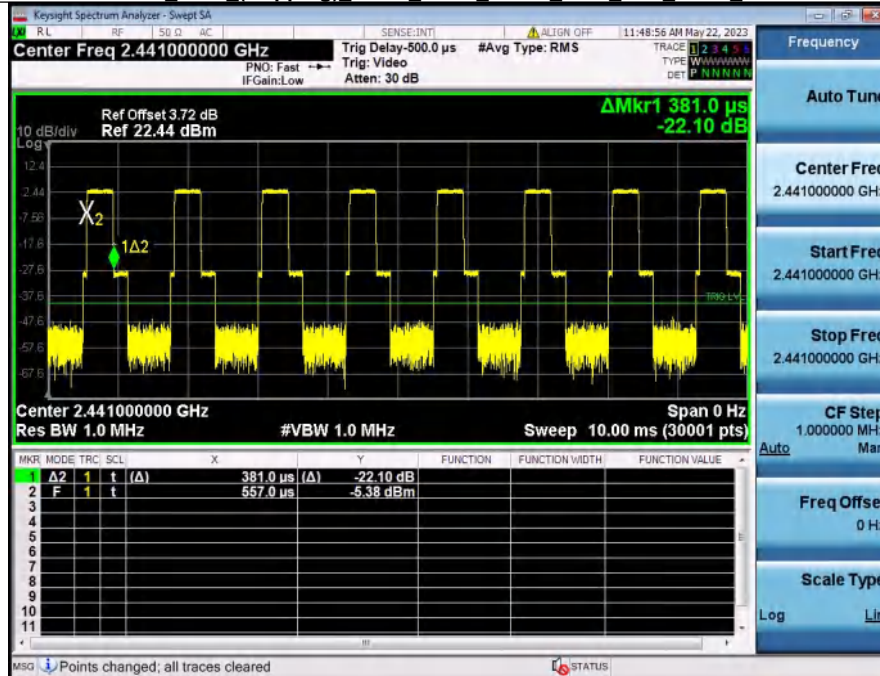
Dwell_Time_(Hopping)_NVNT_ANT1_1-DH1_2441_Accumulated
