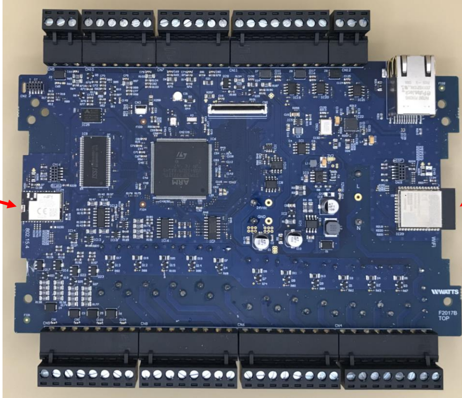
PCB – Top side
