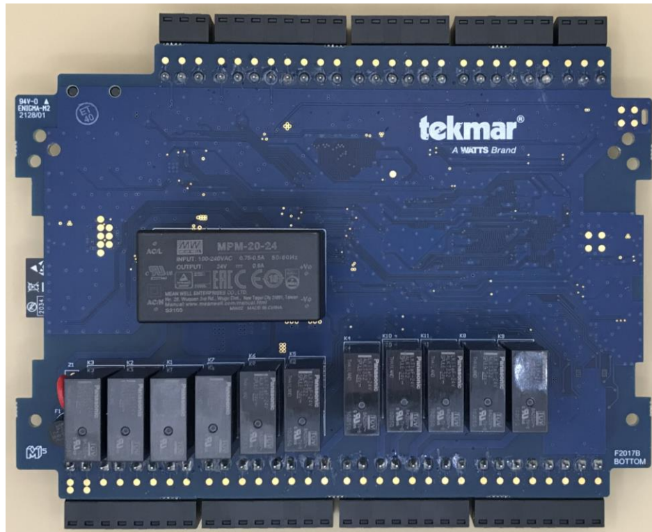
PCB – Bottom side
