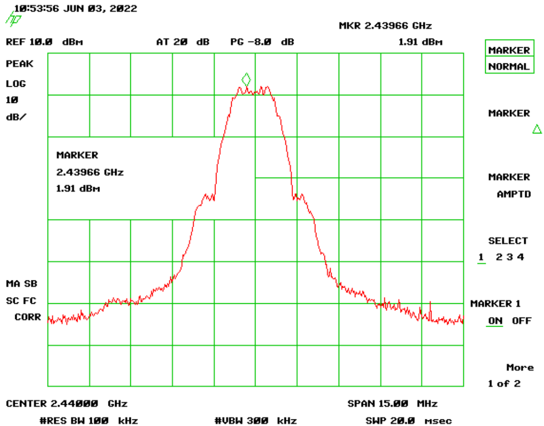
Figure 37. Power Spectral Density, Mid Channel
