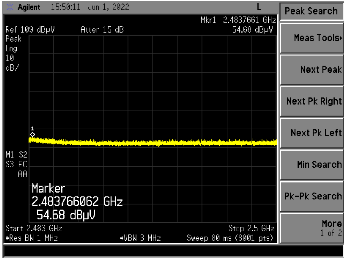
Figure 25. High Channel Restricted Band – Peak (Vertical)
