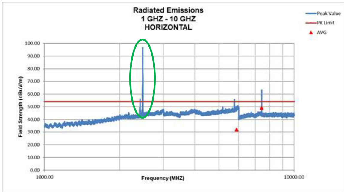
Figure 44. Radiated Emissions, Horizontal 1 GHz – 10 GHz
