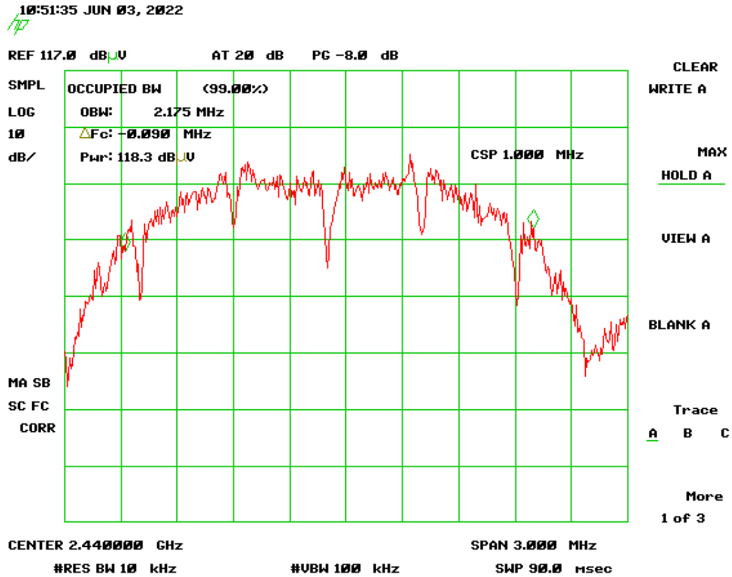
Figure 31. 99% Occupied Bandwidth Mid Channel
