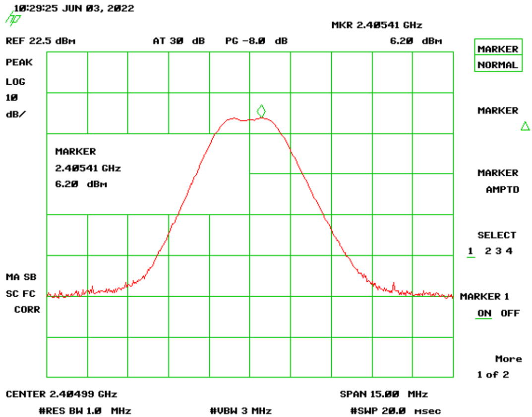
Figure 33. Peak Antenna Conducted Output Power, Low Channel
