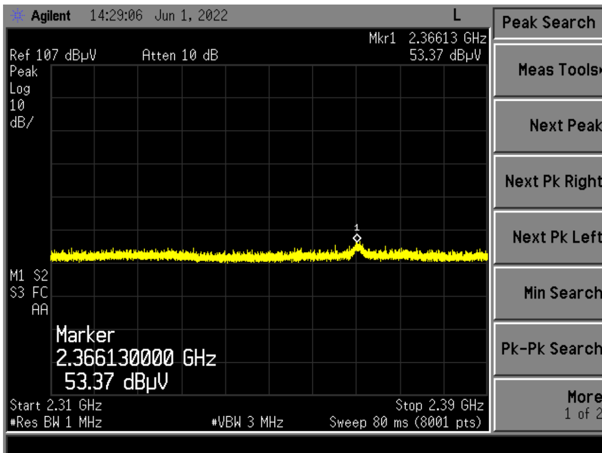
Figure 21. Low Channel Restricted Band – Peak (Vertical)
