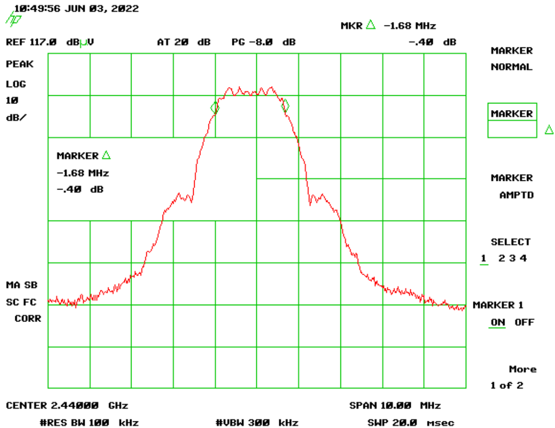
Figure 28. 6 dB Bandwidth Mid Channel
