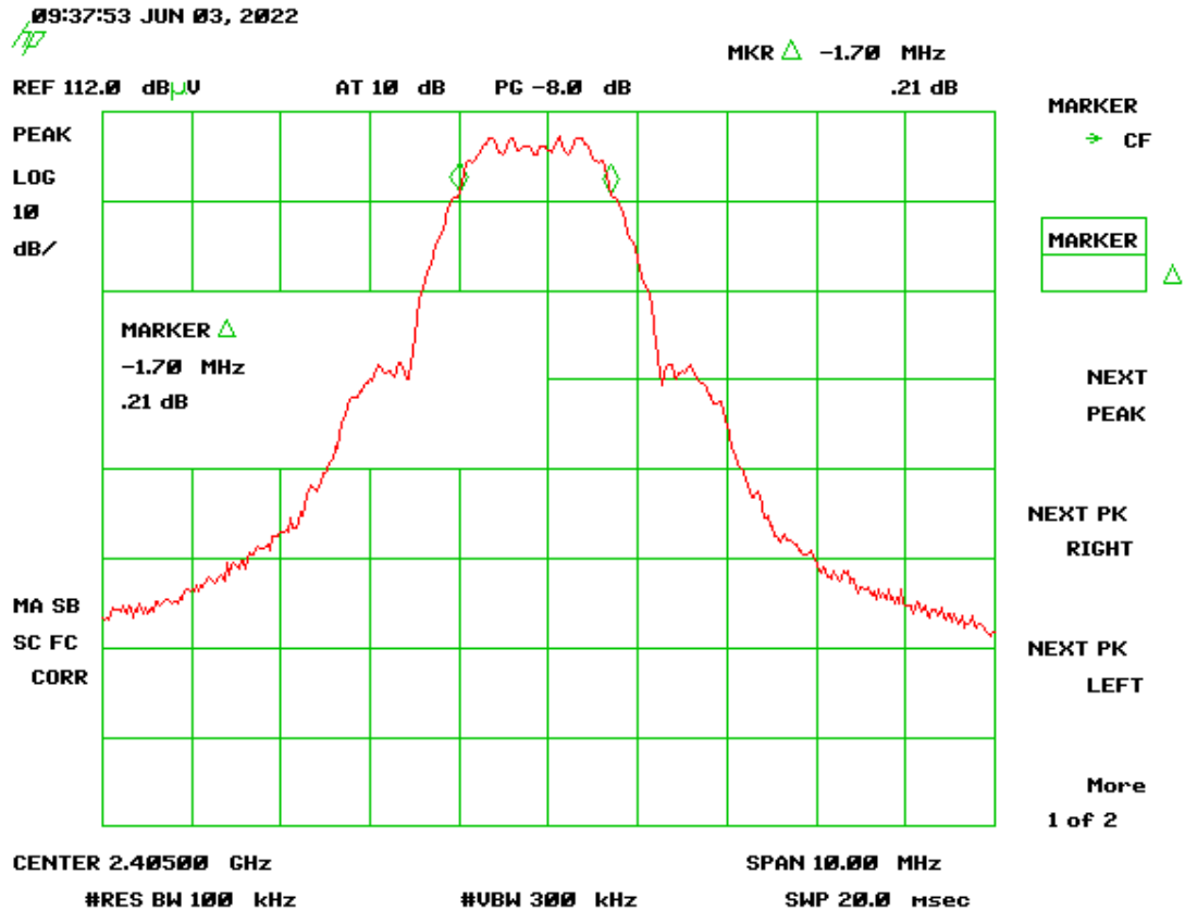
Figure 27. 6 dB Bandwidth Low Channel
