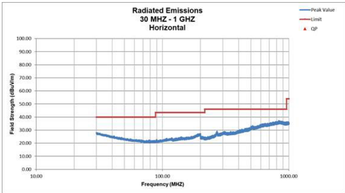
Figure 42. Radiated Emissions, Horizontal 30 MHz – 1 GHz
