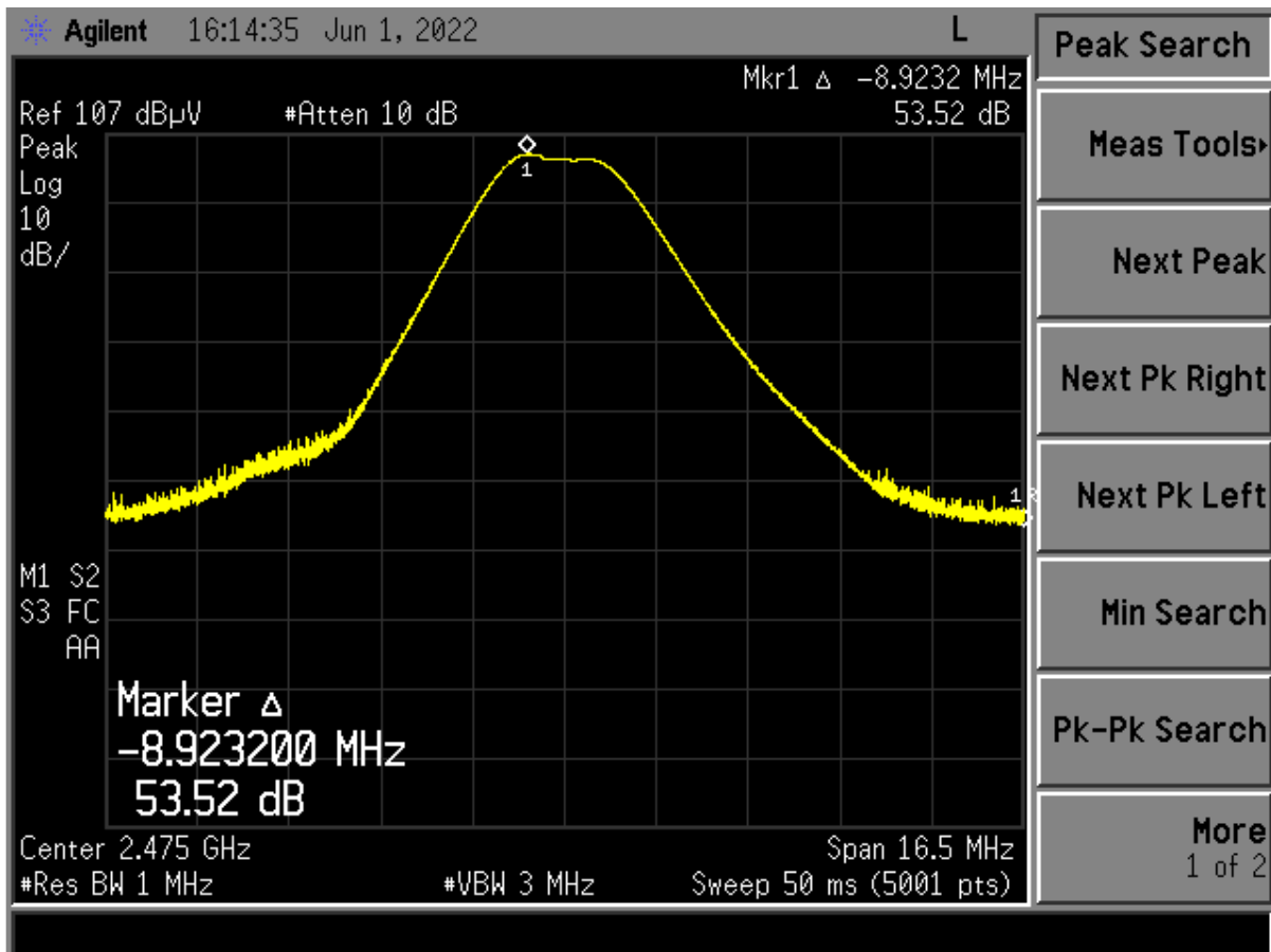
Figure 22. Band Edge Compliance – High Channel Delta – Peak (Horizontal)
