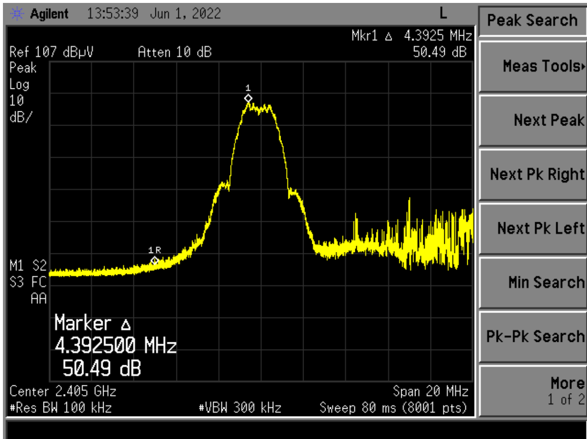
Figure 18. Band Edge Compliance – Low Channel Delta – Peak (Horizontal)
