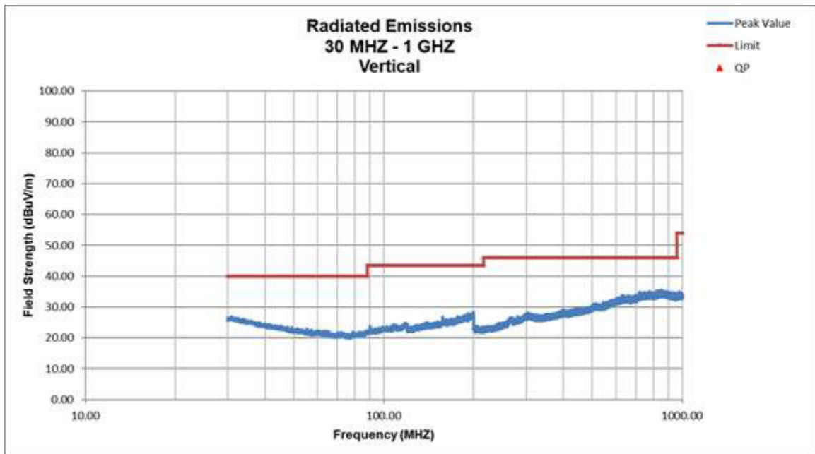
Figure 43. Radiated Emissions, Vertical 30 MHz – 1 GHz
