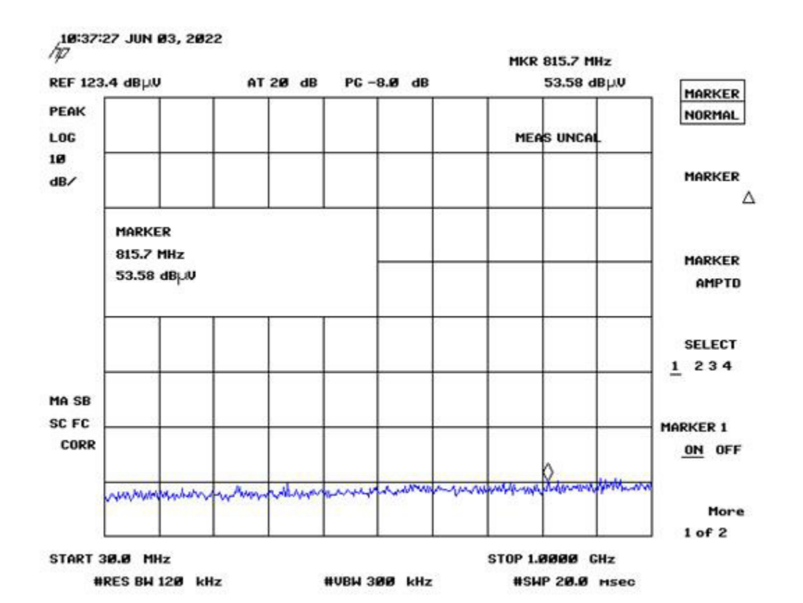
Figure 3. Channel 11, 30-1000 MHz
