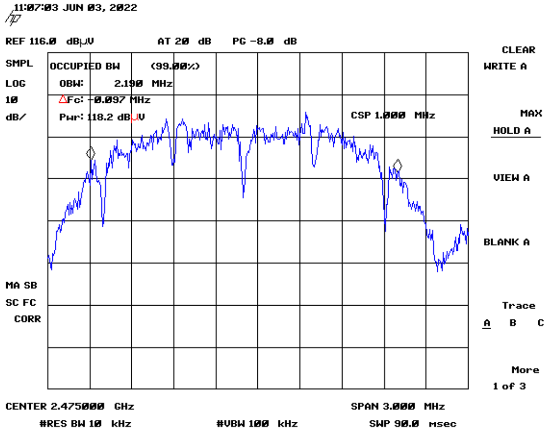
Figure 32. 99% Occupied Bandwidth High Channel
