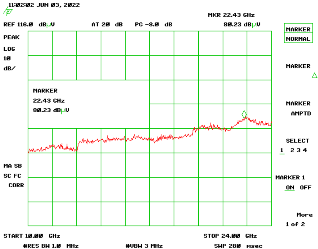
Figure 11. Channel 18, 10-24 GHz
