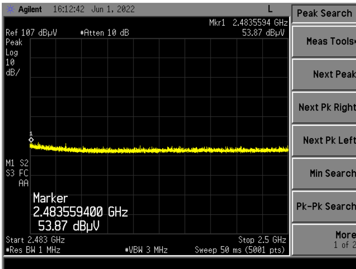
Figure 24. High Channel Restricted Band – Peak (Horizontal)
