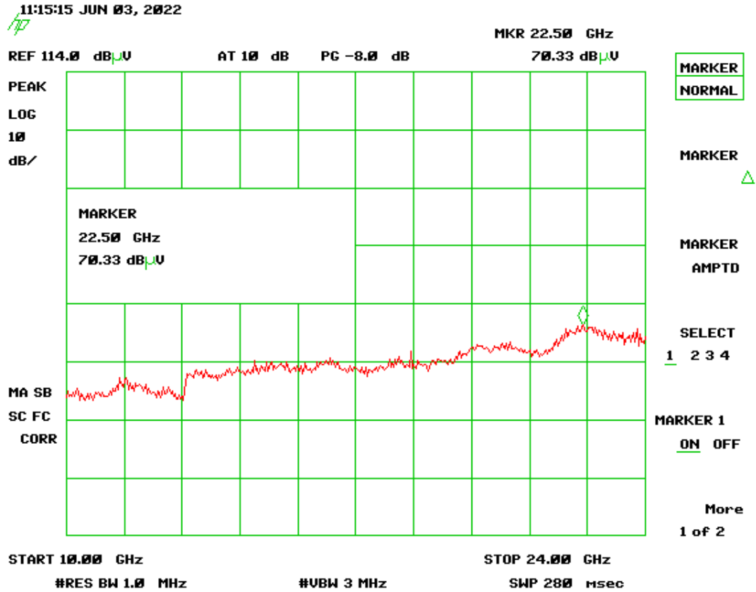
Figure 16. Channel 25, 10-24 GHz
