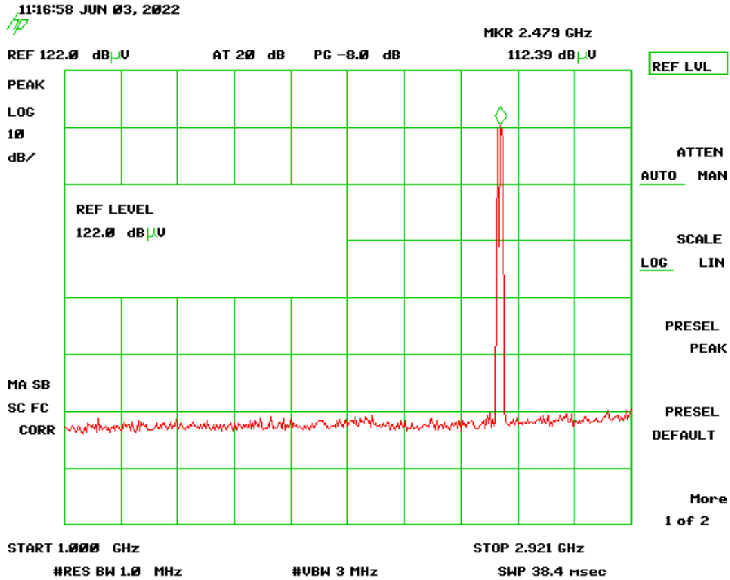
Figure 13. Channel 25, 1 – 2.921 GHz
