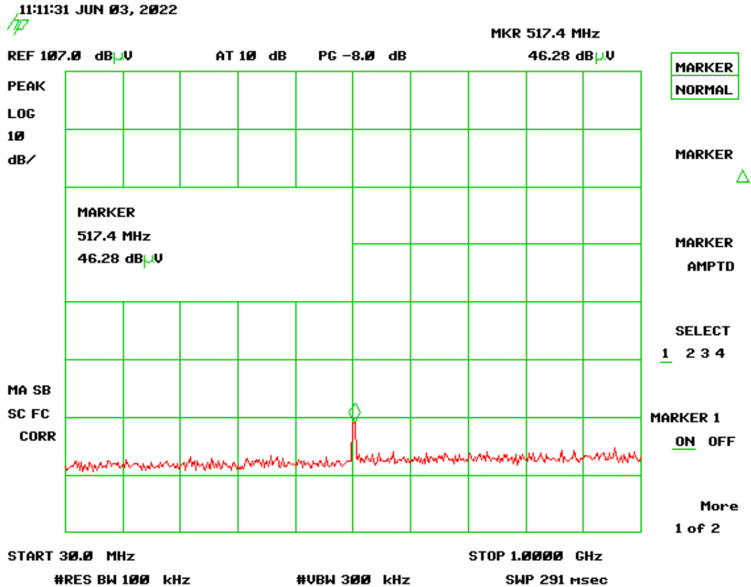
Figure 12. Channel 25, 30-1000 MHz
