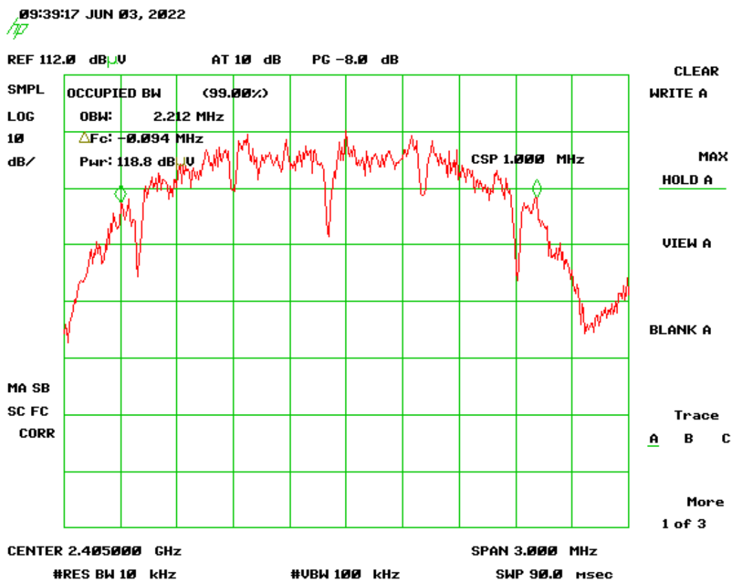
Figure 30. 99% Occupied Bandwidth Low Channel
