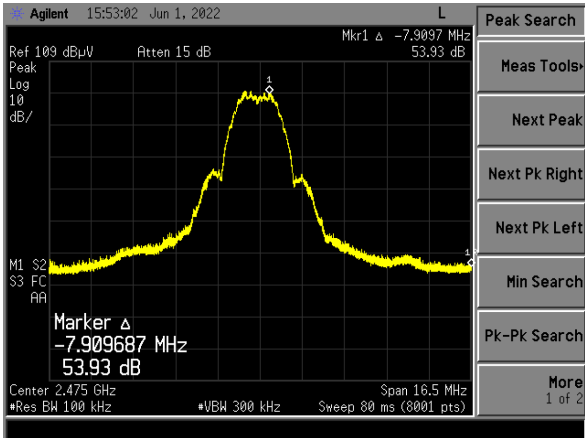
Figure 23. Band Edge Compliance – High Channel Delta – Peak (Vertical)
