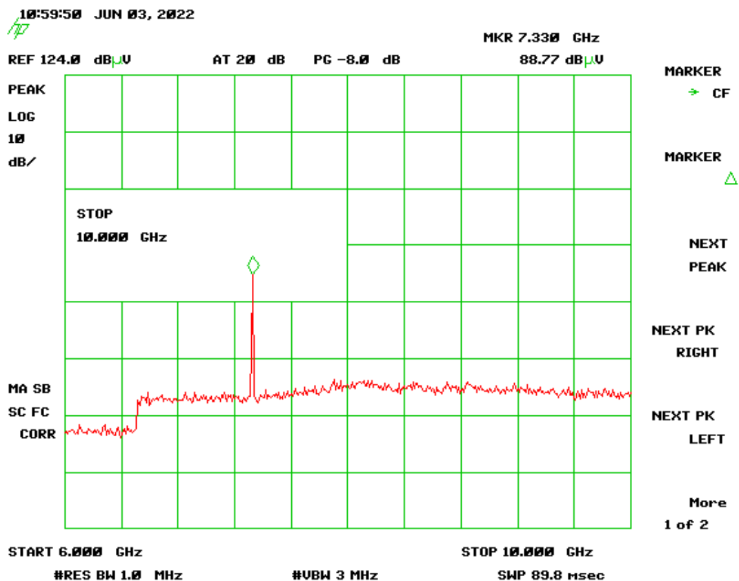
Figure 10. Channel 18, 6-10 GHz
