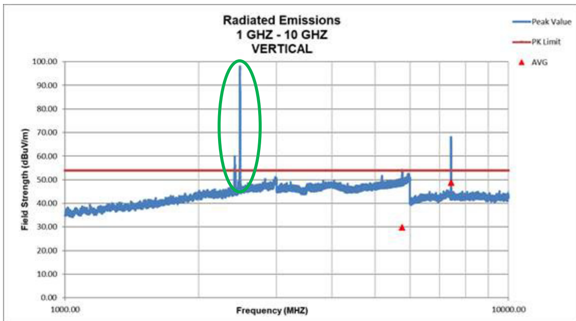
Figure 45. Radiated Emissions, Vertical 1 GHz – 10 GHz
