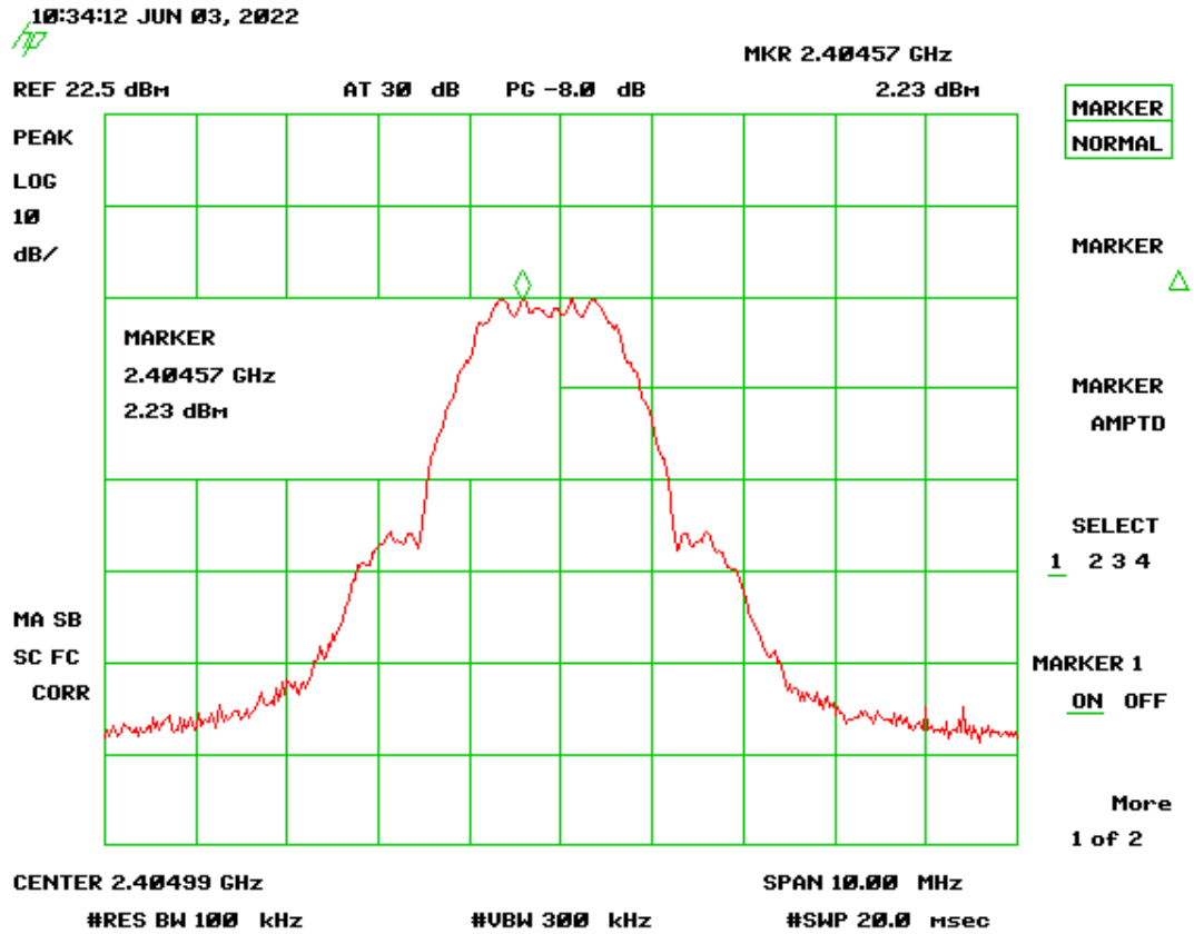
Figure 36. Power Spectral Density, Low Channel
