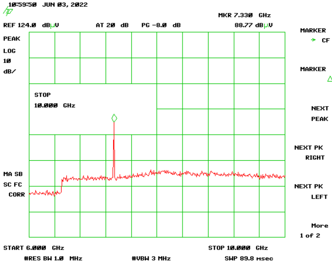
Figure 15. Channel 25, 6-10 GHz
