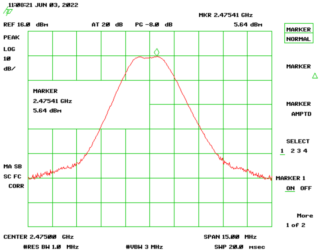
Figure 35. Peak Antenna Conducted Output Power, High Channel
