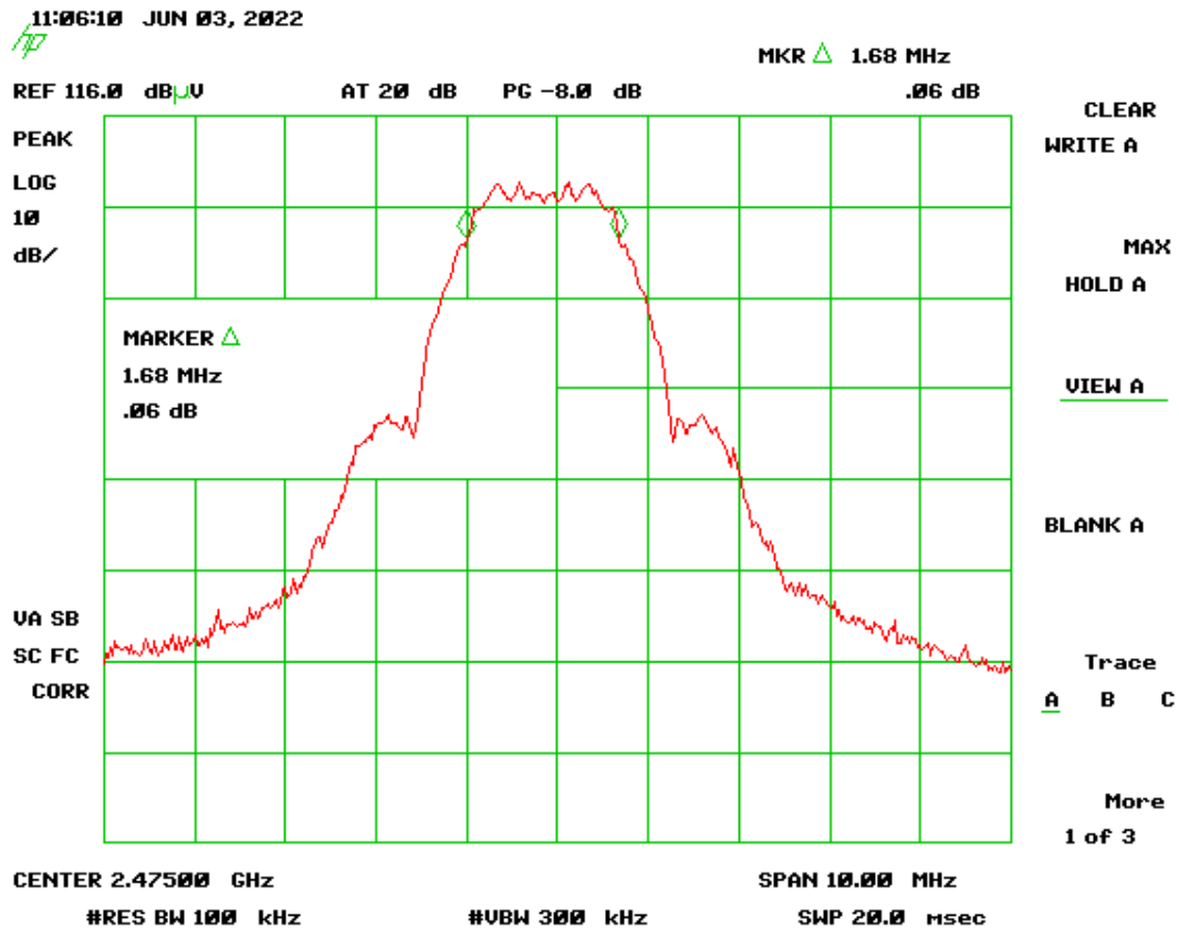
Figure 29. 6 dB Bandwidth High Channel
