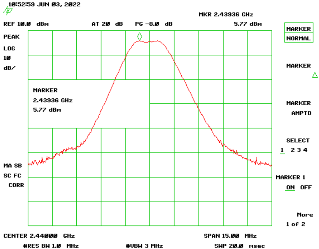
Figure 34. Peak Antenna Conducted Output Power, Mid Channel
