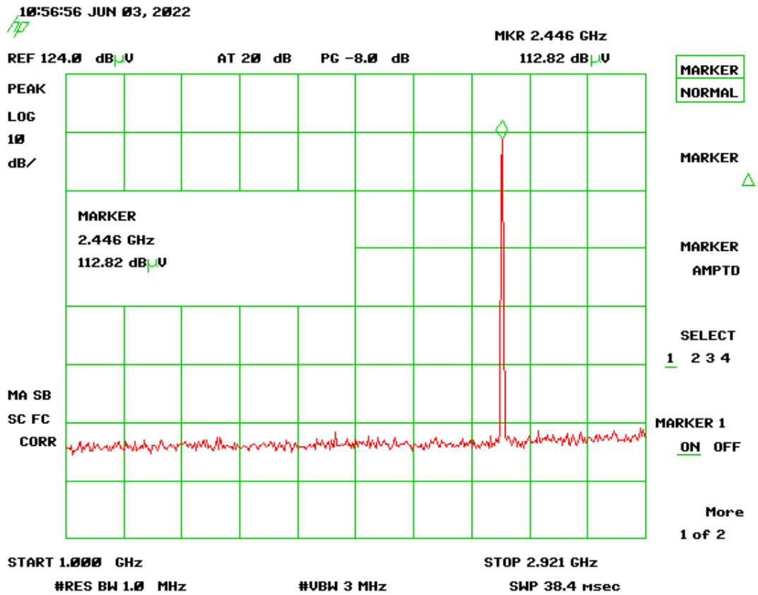
Figure 8. Channel 18, 1-2.921 GHz
