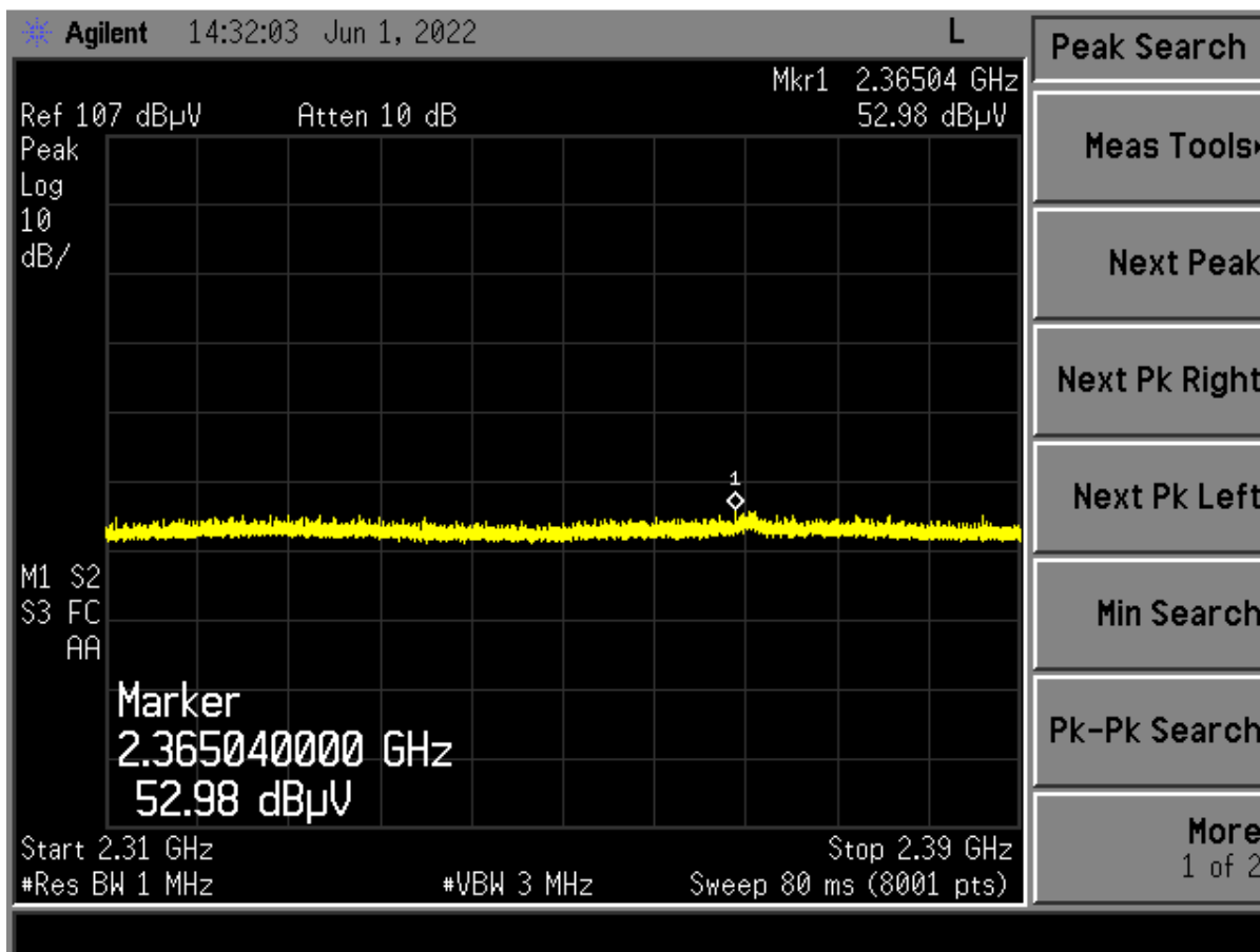
Figure 20. Low Channel Restricted Band – Peak (Horizontal)
