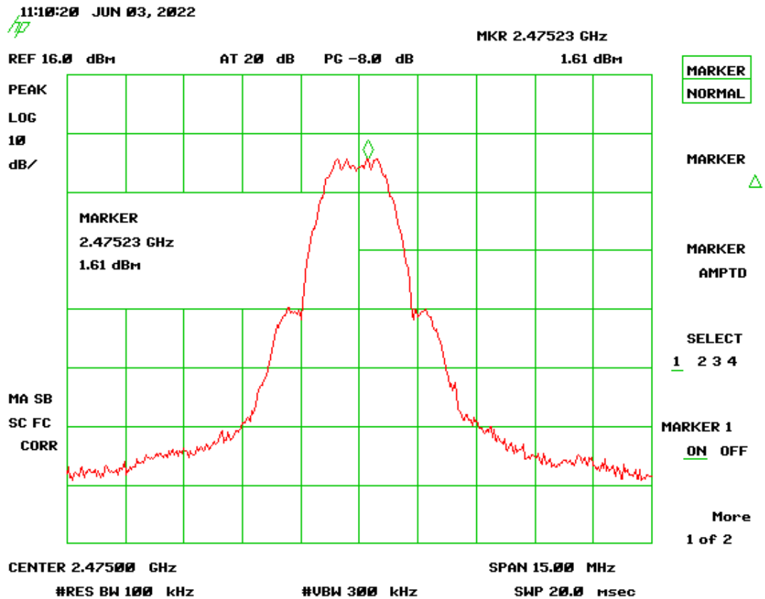
Figure 38. Power Spectral Density, High Channel
