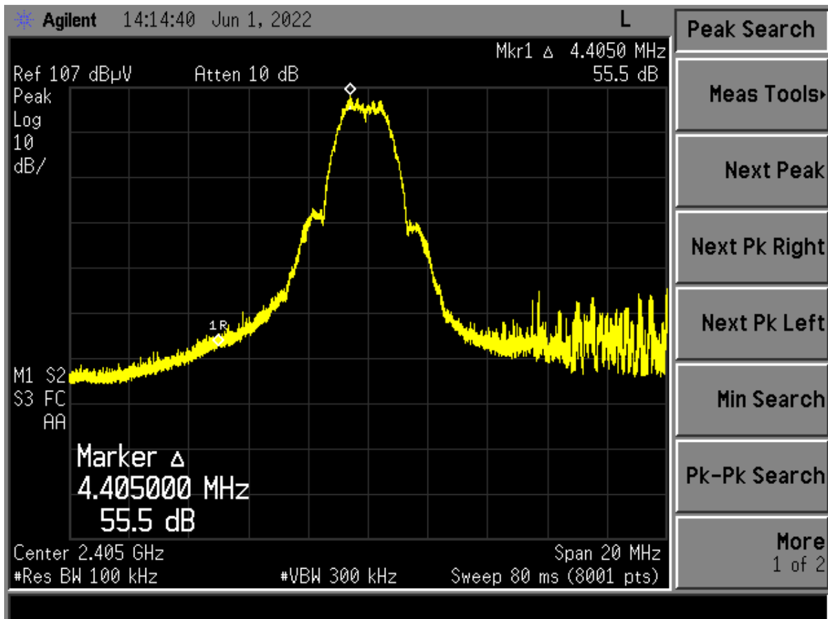
Figure 19. Band Edge Compliance – Low Channel Delta – Peak (Vertical)
