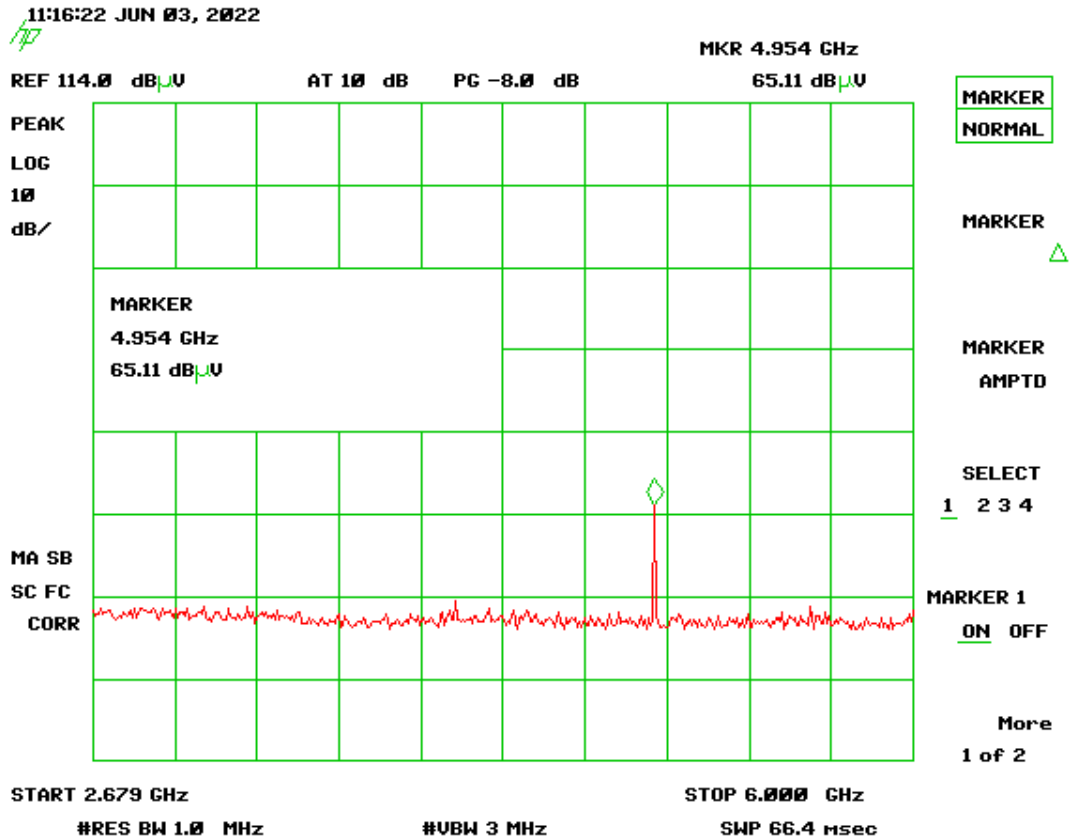
Figure 14. Channel 25, 2.679-6 GHz
