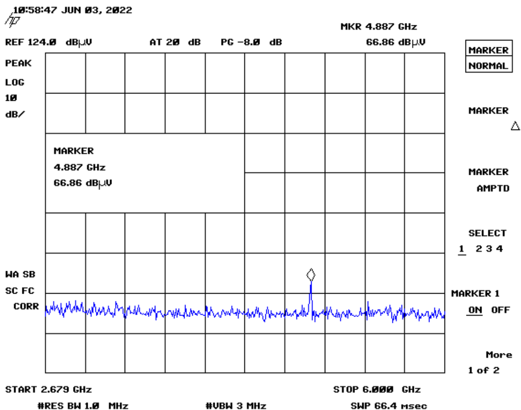
Figure 9. Channel 18, 2.6-6 GHz
