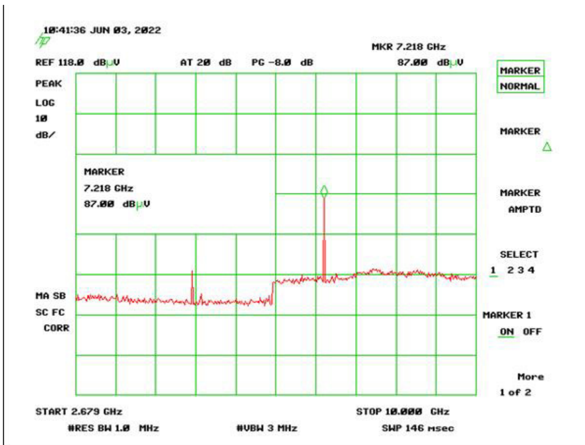
Figure 5. Channel 11, 2.679 - 10 GHz
