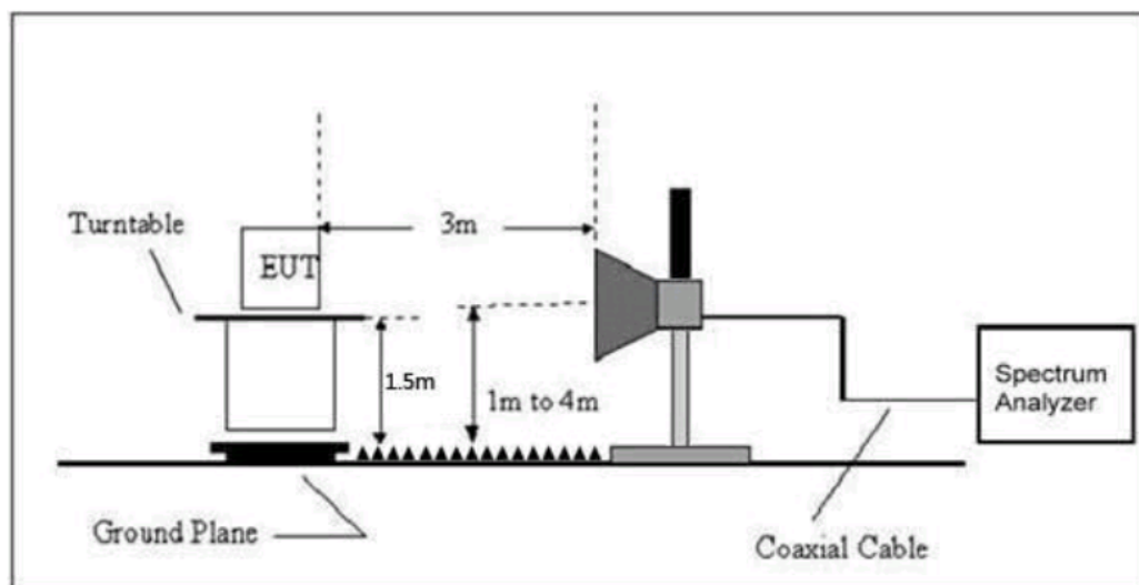
Figure 17. Above 1 GHz Radiated Emissions Test Setup
