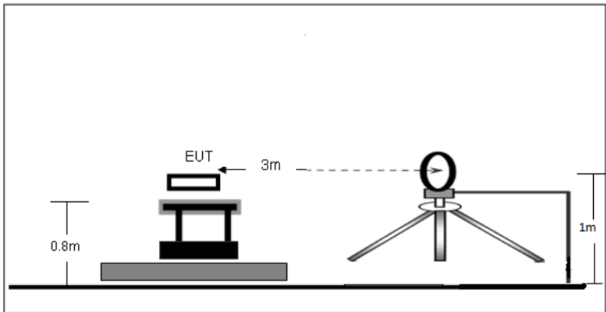
Figure 39. Block Diagram Below 30 MHz Radiated Emissions Test Setup
