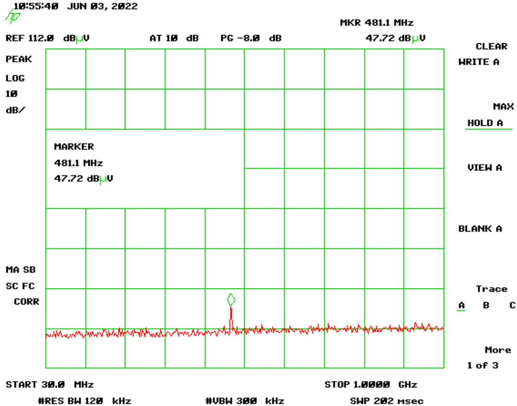
Figure 7. Channel 18, 30-1000 MHz
