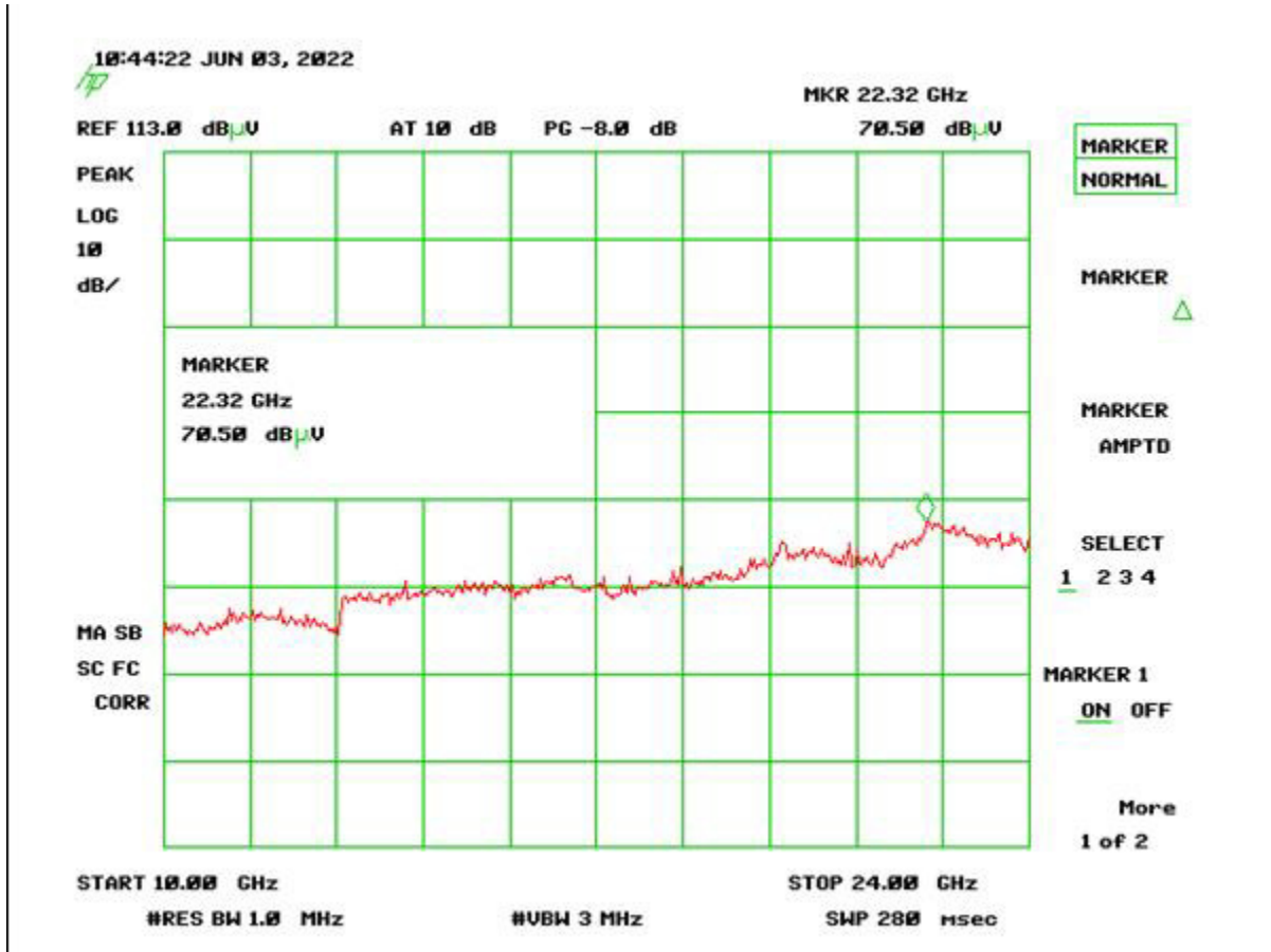
Figure 6. Channel 11, 10-24 GHz
