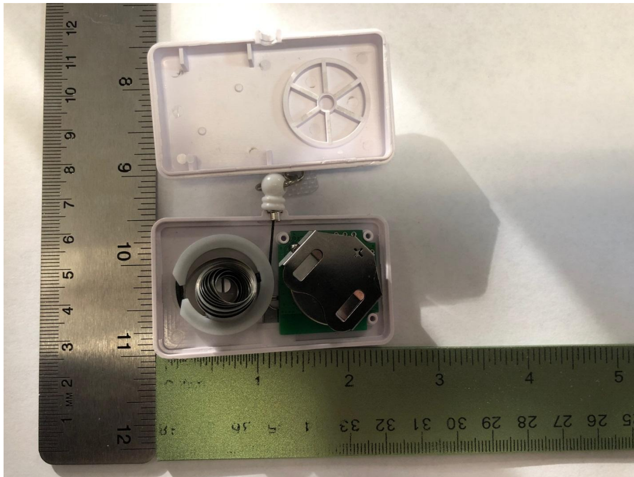
Figure 1. EUT, Inside View
