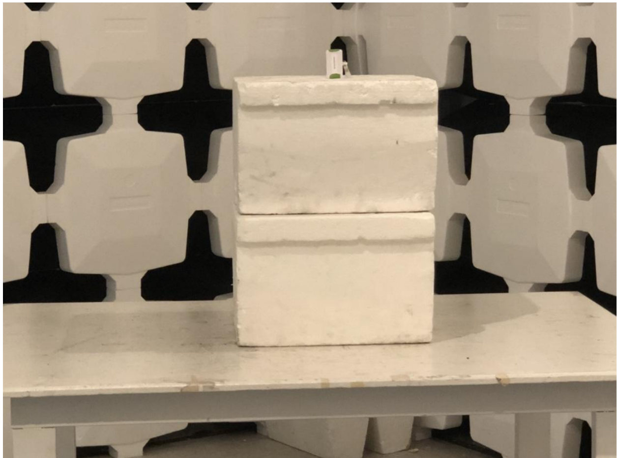
Figure 1. EUT Radiated Emissions Test Setup
