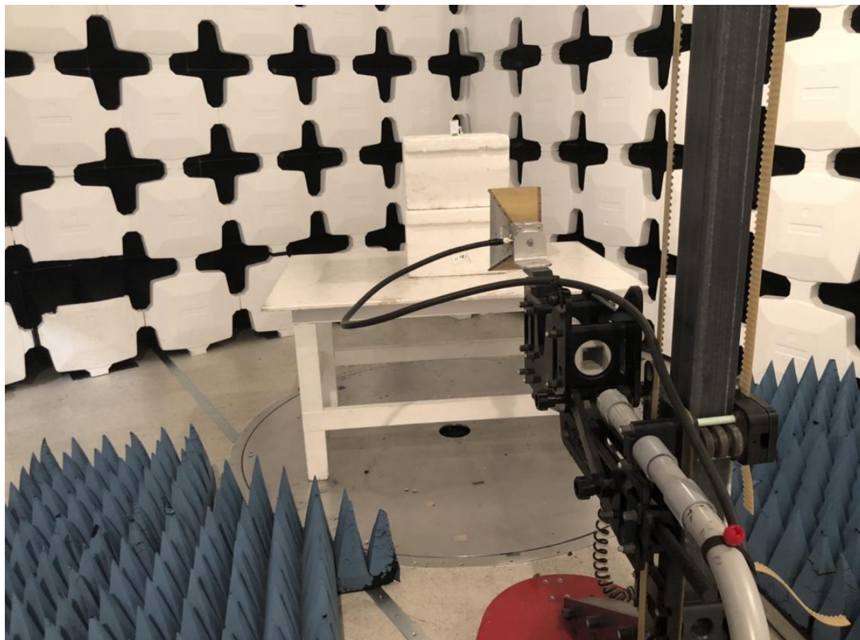
Figure 6. Radiated Emissions, > 6 GHz
