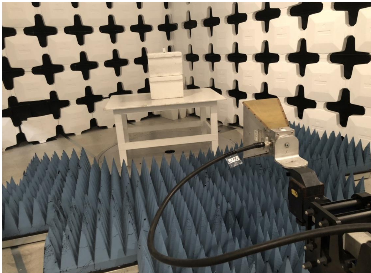
Figure 5. Radiated Emissions, 1 - 6 GHz
