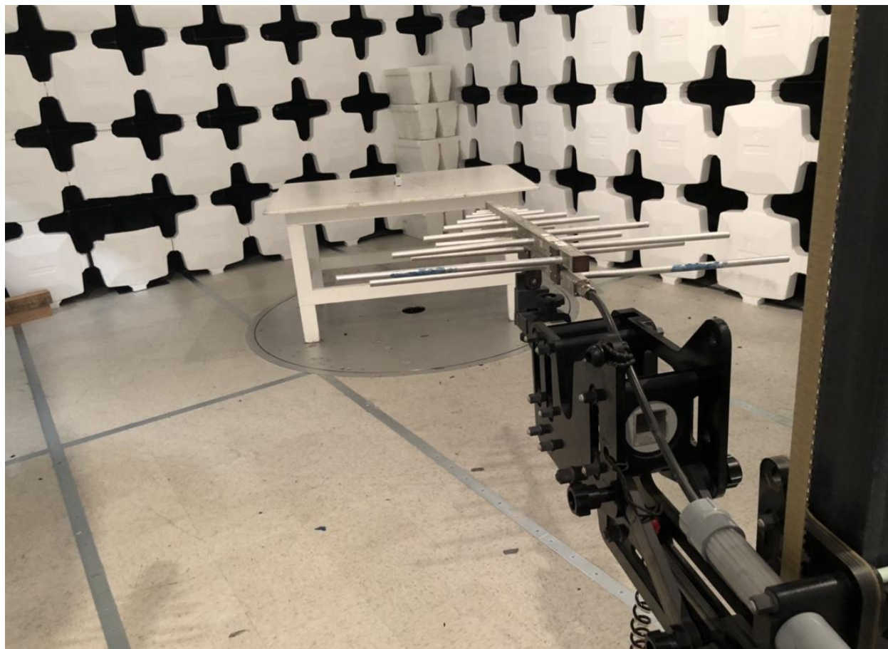
Figure 4. Radiated Emissions, 200-1000 MHz
