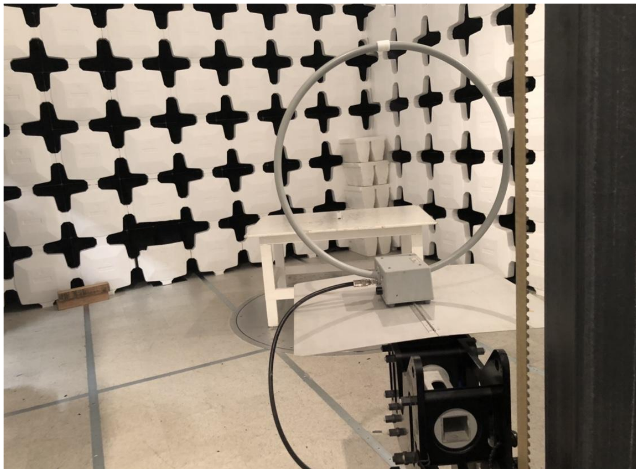
Figure 2. Spurious Radiated Emissions Below 30 MHz, X Polarity
