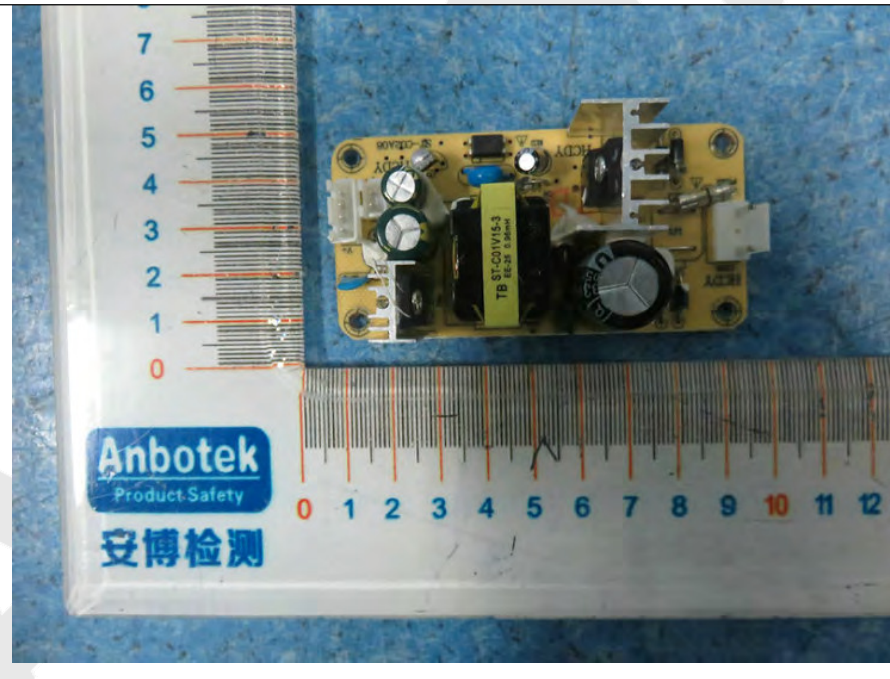
24. Figure PCB of the EUT-Front View
