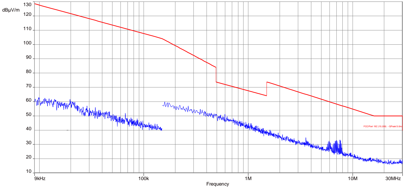
Plot 1: 9 kHz to 30 MHz, GFSK, channel 00, transmit mode
