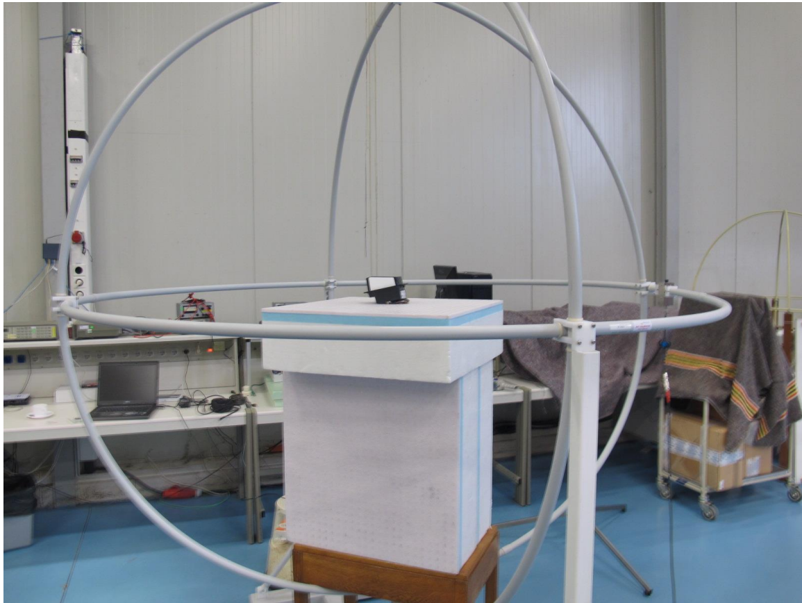
Photograph 1: Equipment under test in large loop antenna system (0.009 - 30 MHz)
