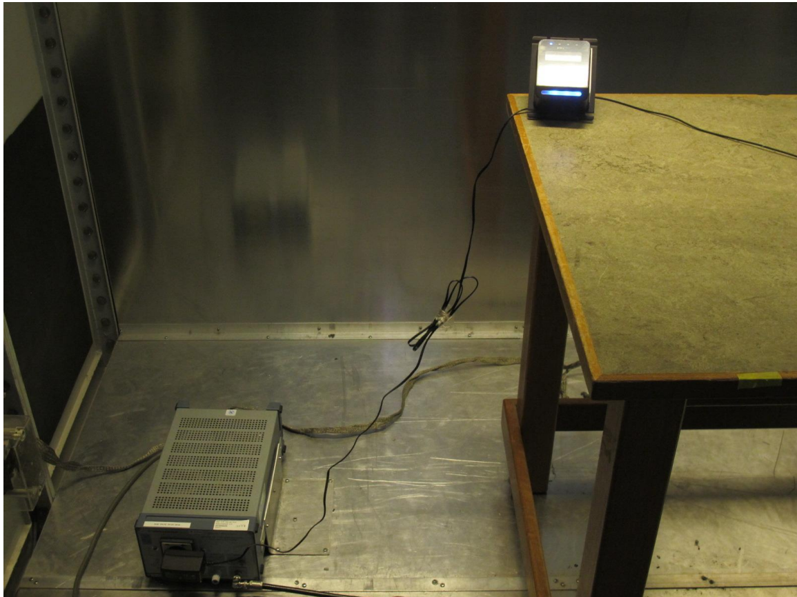
Photograph 3: Equipment under test in Conducted Emissions test room (0.15 – 30 MHz)
