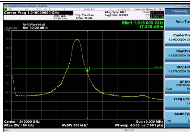
HighRange_FDD25_5MHz_1912.5_fullRB_High_Q16
