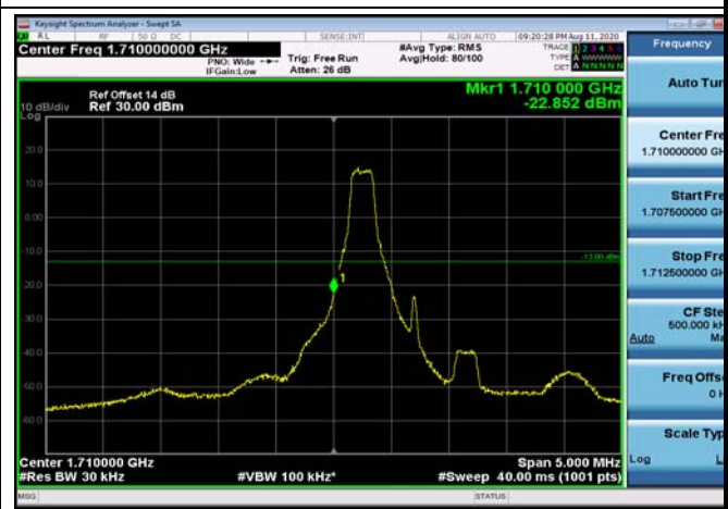
LowRange_FDD66_1.4MHz_1710.7_OneRB _low_Q16
