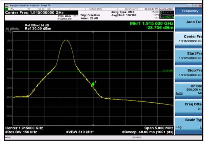
HighRange_FDD25_15MHz_1907.5_OneRB _high_Q16
