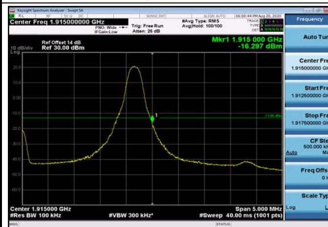
HighRange_FDD25_5MHz_1912.5_fullRB_High_QPSK
