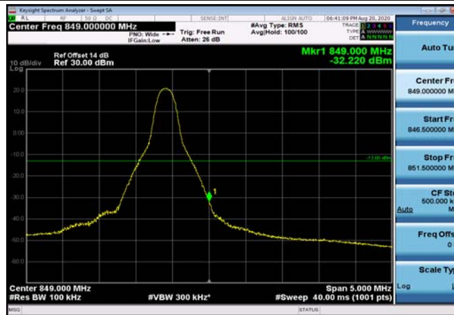
HighRange_FDD26_10MHz_844_fullRB _High_QPSK
