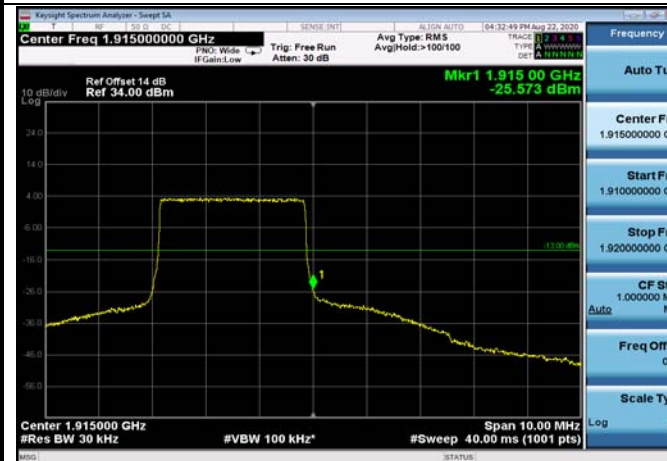
HighRange_FDD25_5MHz_1912.5_OneRB_high_QPSK
