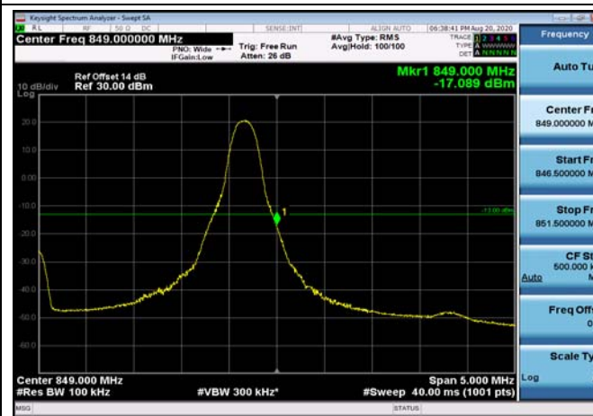
HighRange_FDD26_5MHz_846.5_OneRB _high_QPSK
