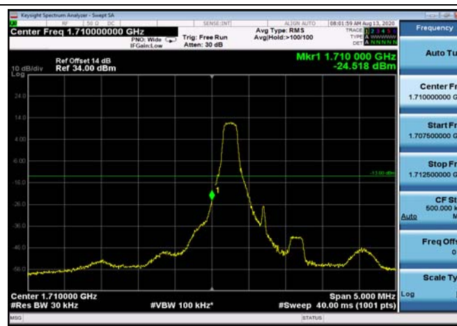
LowRange_FDD66_1.4MHz_1710.7_OneRB _low_QPSK
