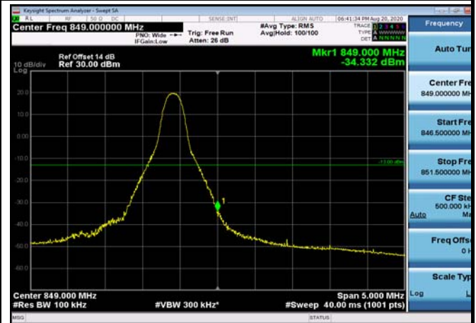
HighRange_FDD26_10MHz_844_fullRB _High_Q16
