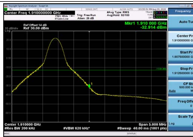
HighRange_FDD02_20MHz_1900_OneRB _high_QPSK
