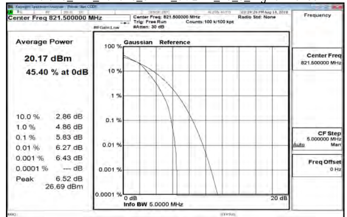
Part 90_LTE_Band26_5MHz_64QAM_25_0_HighCH26765
