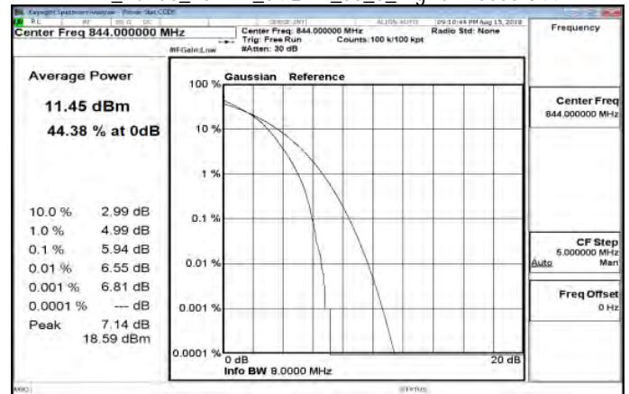
LTE_Band5_10MHz_64QAM_50_0_HighCH20600-844
