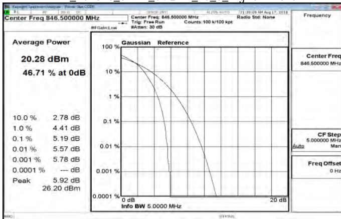
LTE_Band26_5MHz_64QAM_25_0_HighCH27015
