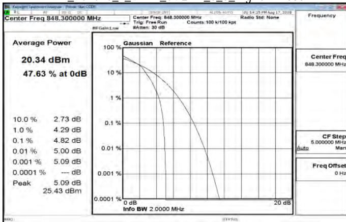
LTE_Band26_1_4MHz_64QAM_6_0_HighCH27033
