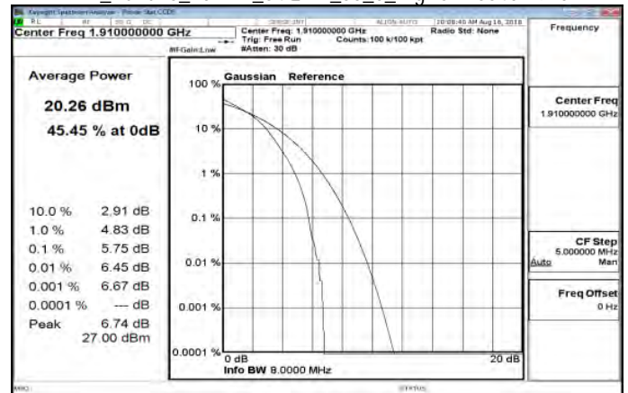
LTE_Band25_10MHz_64QAM_50_0_HighCH26640-1910
