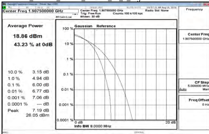
LTE_Band25_15MHz_64QAM_75_0_HighCH26615-1907.5
