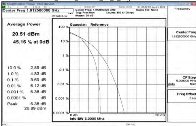
LTE_Band25_5MHz_64QAM_25_0_HighCH26665-1912.5
