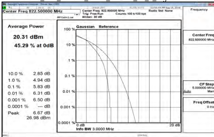
Part 90_LTE_Band26_3MHz_64QAM_15_0_HighCH26775
