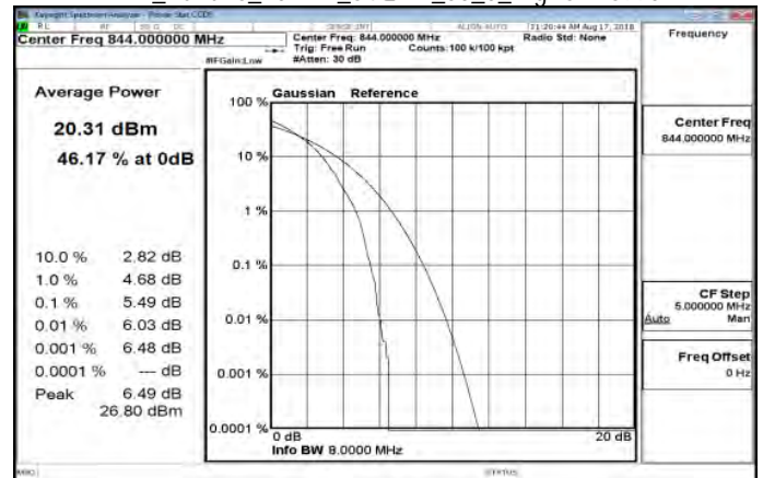
LTE_Band26_10MHz_64QAM_50_0_HighCH26990
