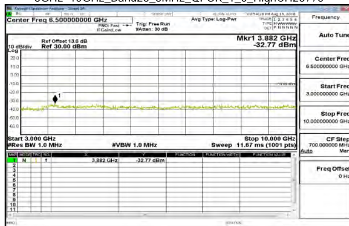
3GHz~10GHz_Band26_3MHz_QPSK_1_0_HighCH26775
