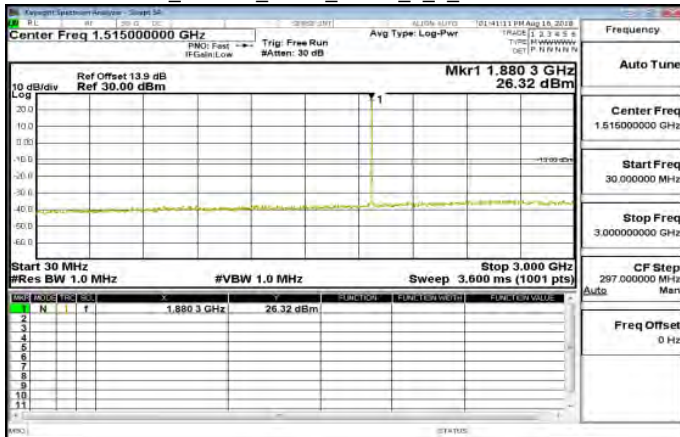
30MHz-3GHz_Band25_3MHz_QPSK_1_0_MidCH26365-1882.5
