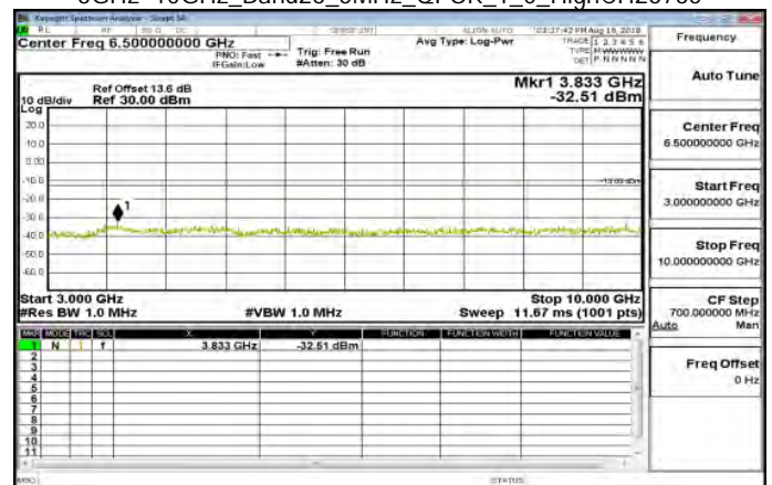
3GHz~10GHz_Band26_5MHz_QPSK_1_0_HighCH26765
