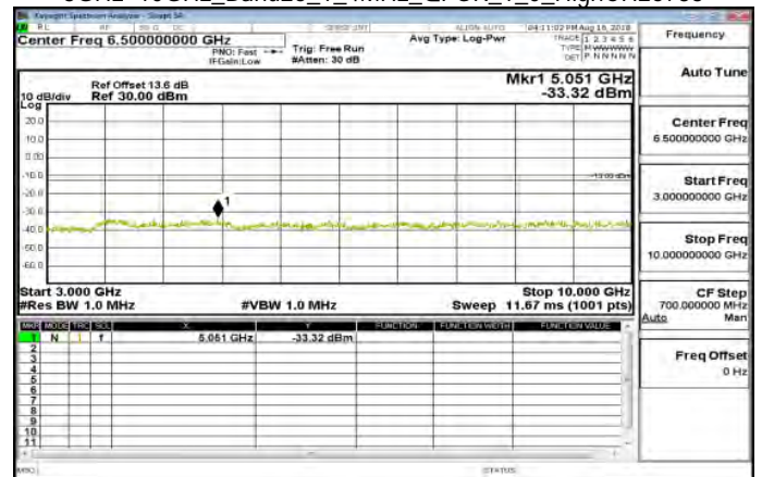
3GHz~10GHz_Band26_1_4MHz_QPSK_1_0_HighCH26783
