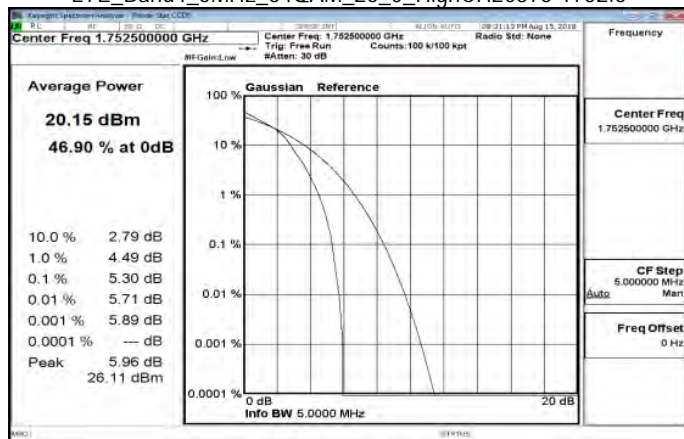
LTE_Band4_5MHz_64QAM_25_0_HighCH20375-1752.5
