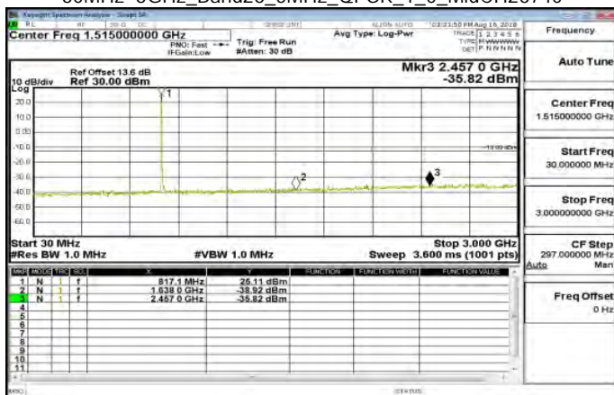
30MHz~3GHz_Band26_5MHz_QPSK_1_0_MidCH26740
