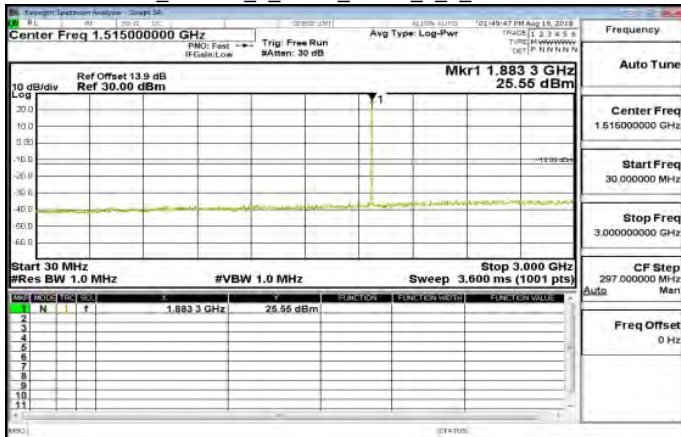
30MHz-3GHz_Band25_1_4MHz_QPSK_1_0_MidCH26365-1882.5
