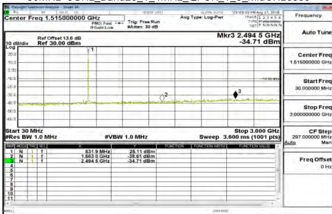
30MHz~3GHz_Band26_1_4MHz_QPSK_1_0_MidCH26865
