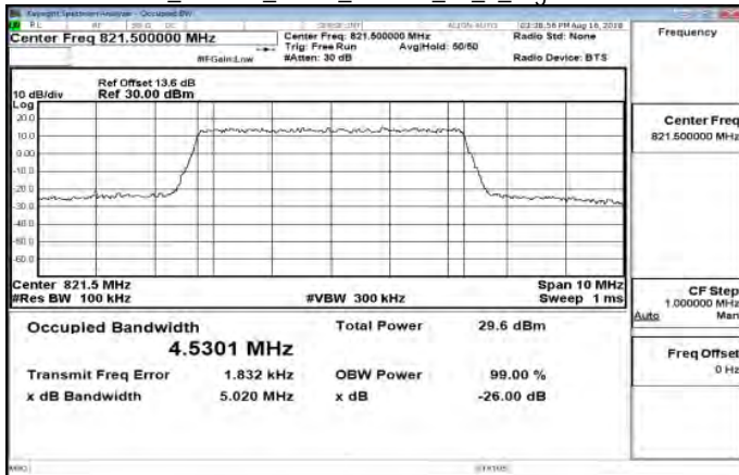
Part 90_Band26_5MHz_16QAM_25_0_HighCH26765
