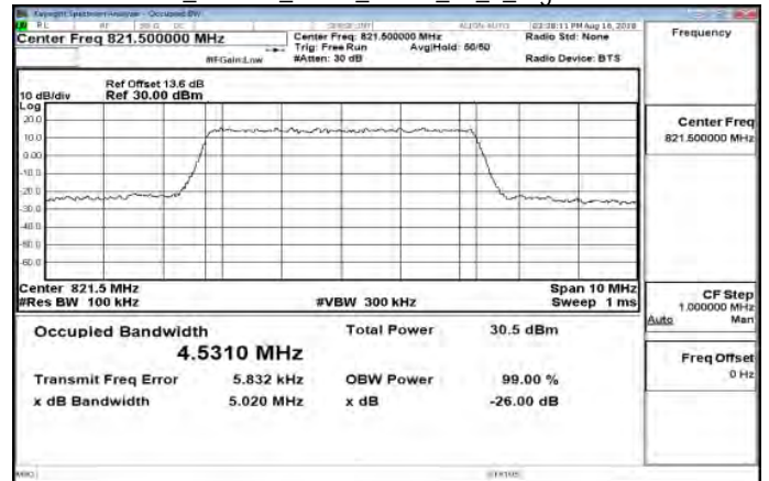
Part 90_Band26_5MHz_QPSK_25_0_HighCH26765
