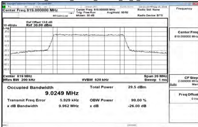
Part 90_Band26_10MHz_64QAM_50_0_MidCH26740
