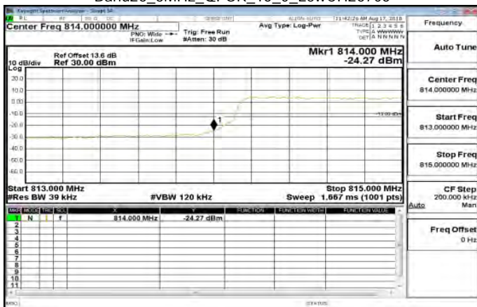
Band26_3MHz_QPSK_15_0_LowCH26705
