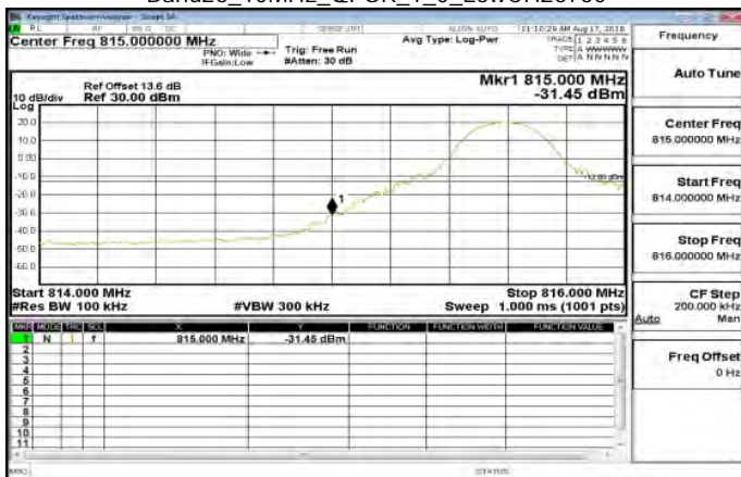
Band26_10MHz_QPSK_1_0_LowCH26750
