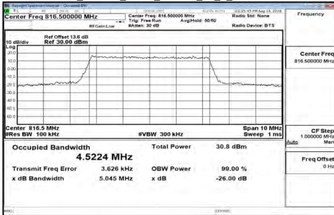
Part 90_Band26_5MHz_16QAM_25_0_MidCH26740
