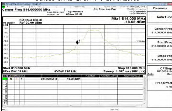
Band26_3MHz_QPSK_1_0_LowCH26705
