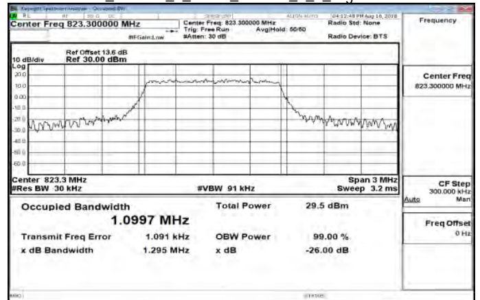
Part 90_Band26_1_4MHz_64QAM_6_0_HighCH26783
