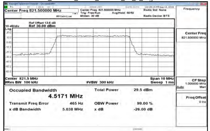
Part 90_Band26_5MHz_64QAM_25_0_HighCH26765
