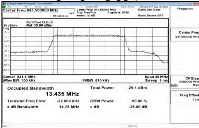
Band26_15MHz_64QAM_75_0_HighCH26965
