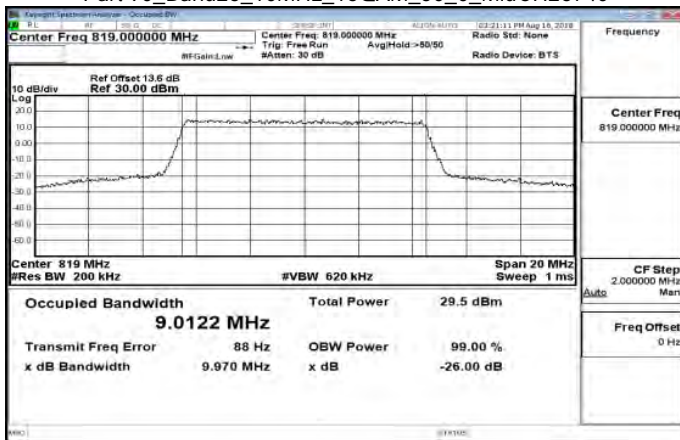
Part 90_Band26_10MHz_64QAM_50_0_MidCH26740
