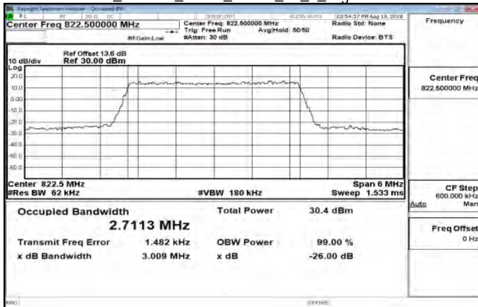
Part 90_Band26_3MHz_QPSK_15_0_HighCH26775
