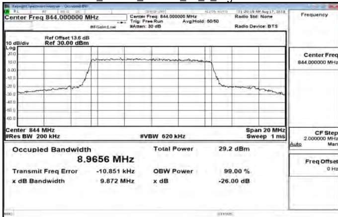
Band26_10MHz_16QAM_50_0_HighCH26990
