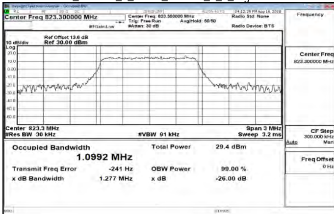
Part 90_Band26_1_4MHz_16QAM_6_0_HighCH26783
