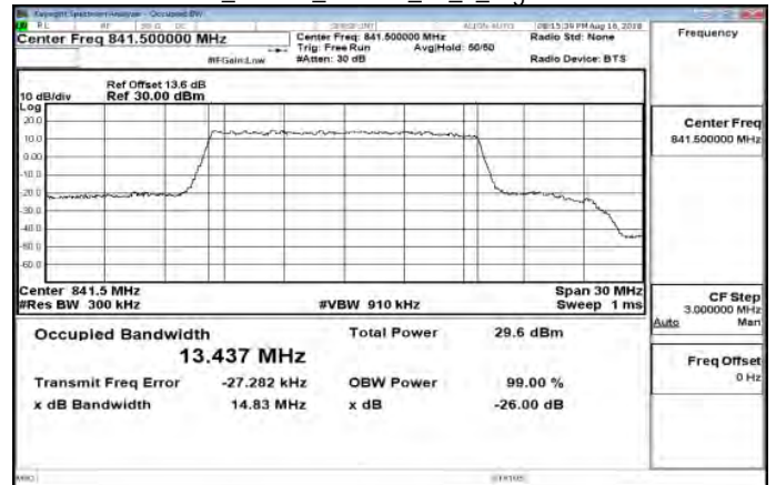
Band26_15MHz_16QAM_75_0_HighCH26965
