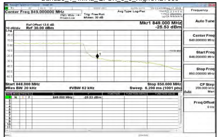
Band26_1_4MHz_QPSK_6_0_HighCH27033
