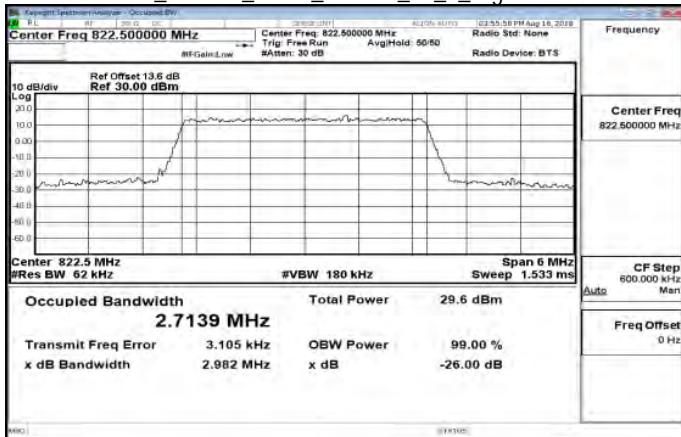
Part 90_Band26_3MHz_64QAM_15_0_HighCH26775
