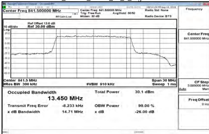
Band26_15MHz_QPSK_75_0_HighCH26965
