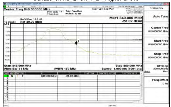
Band26_5MHz_QPSK_1_24_HighCH27015
