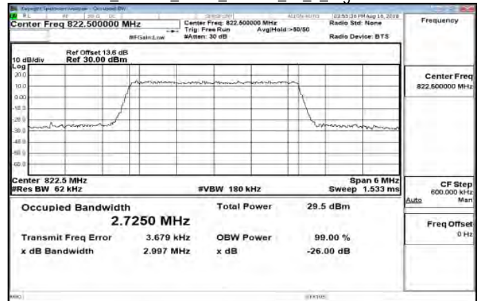
Part 90_Band26_3MHz_16QAM_15_0_HighCH26775
