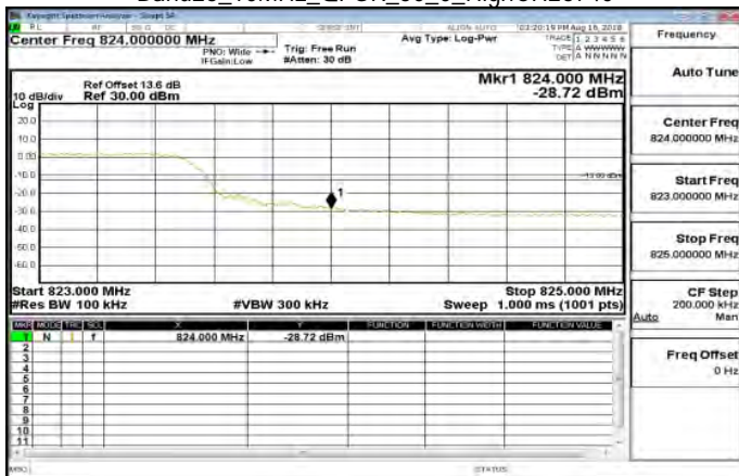
Band26_10MHz_QPSK_50_0_HighCH26740
