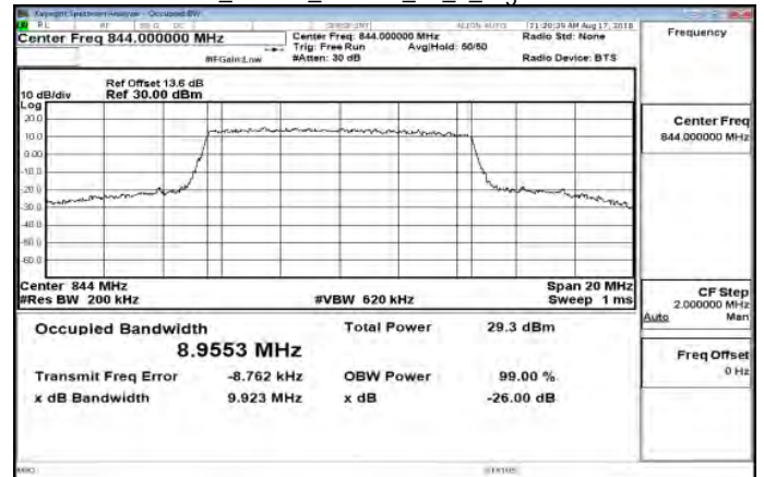
Band26_10MHz_64QAM_50_0_HighCH26990
