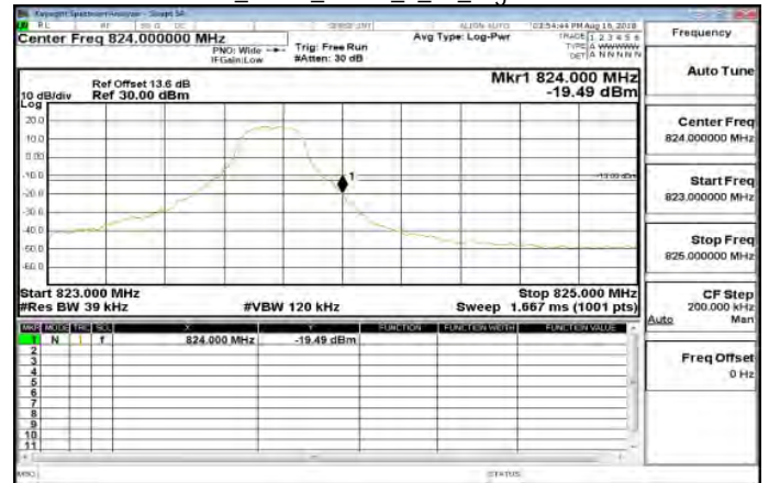
Band26_3MHz_QPSK_15_0_LowCH26705
