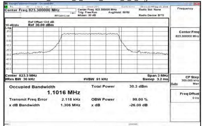
Part 90_Band26_1_4MHz_QPSK_6_0_HighCH26783
