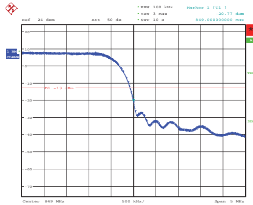
Channel – QPSK
