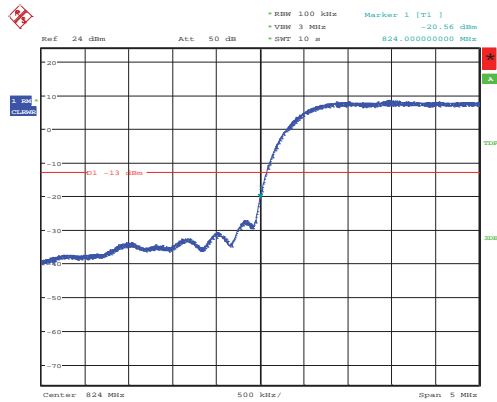
Channel 4132 – QPSK
