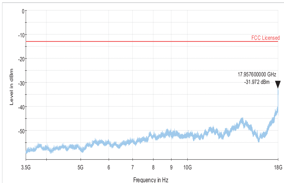
3.5 GHz – 18 GHz
