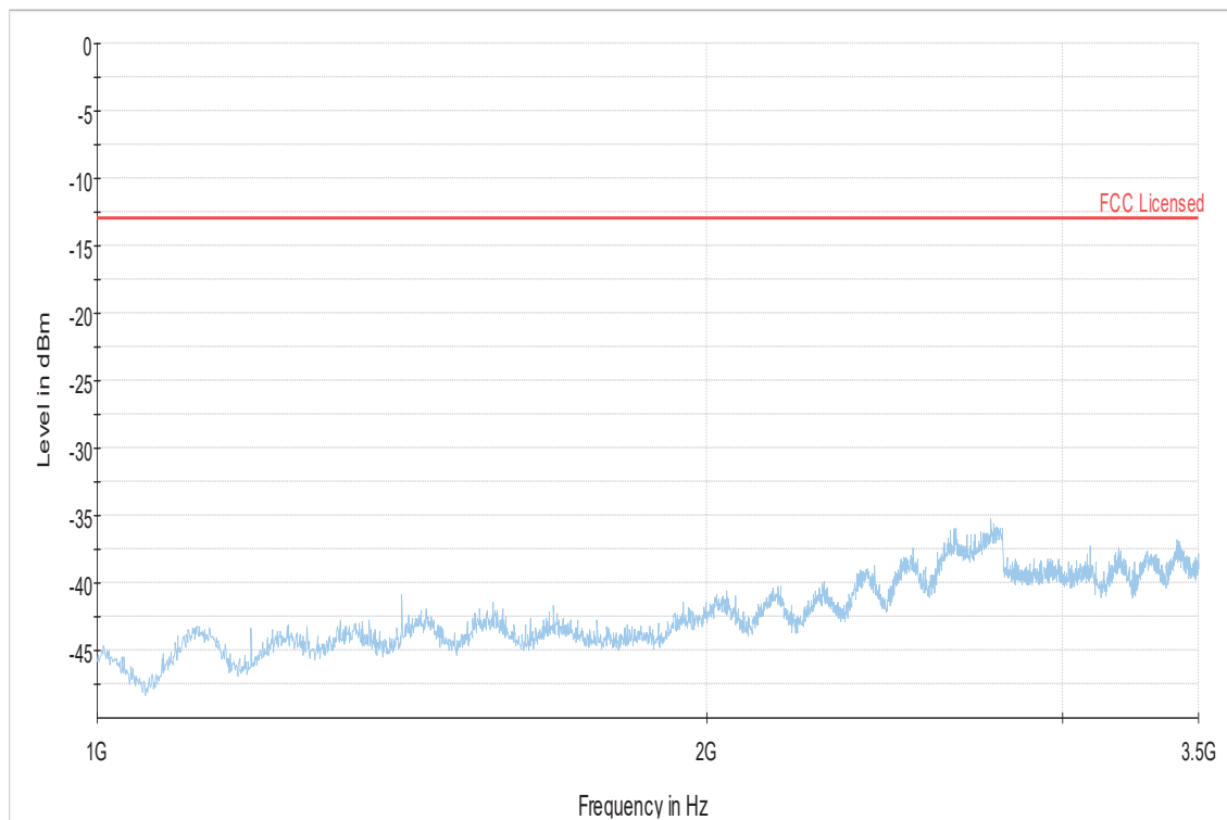
1 GHz – 3.5 GHz
