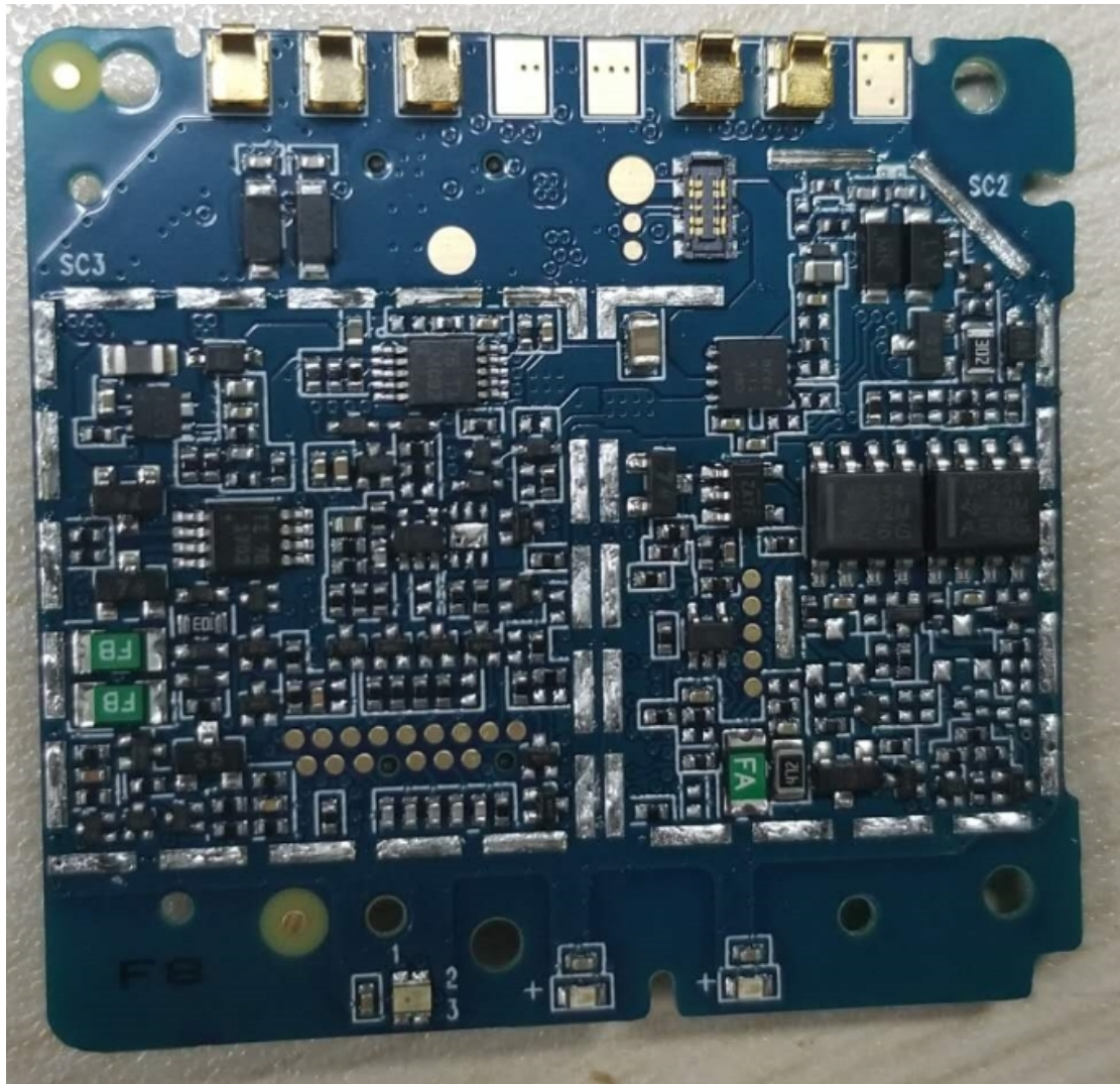
A side of OBD board
