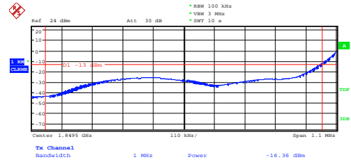
Integration 1 MHz outside the authorized band
