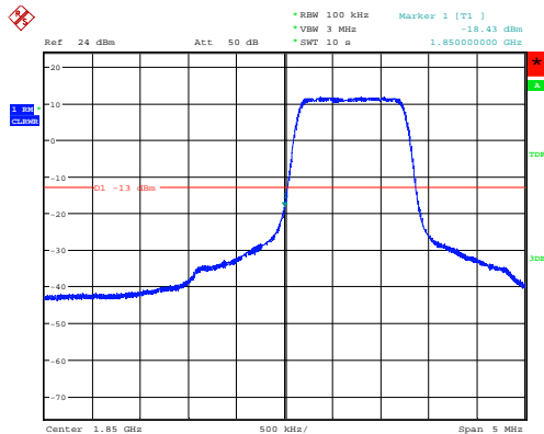
1.4 MHz – Ch: 18607 – RB# 6 RB Pos: 0
