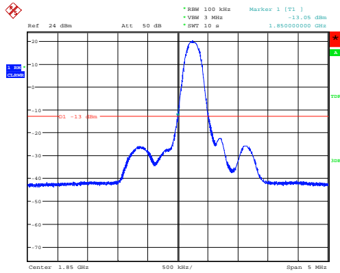
1.4 MHz – Ch: 18607 – RB# 1 RB Pos: 0
