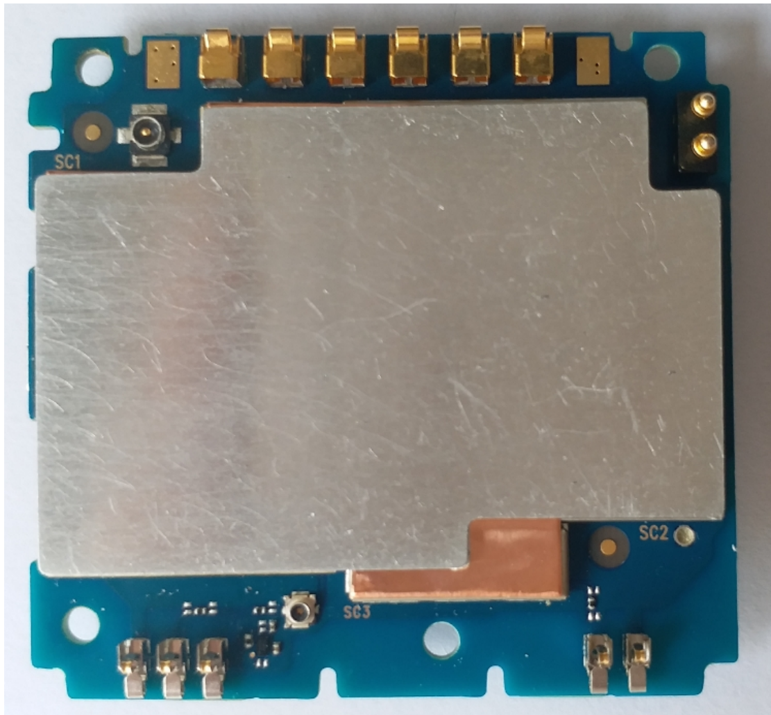
A side of RF board with shield
