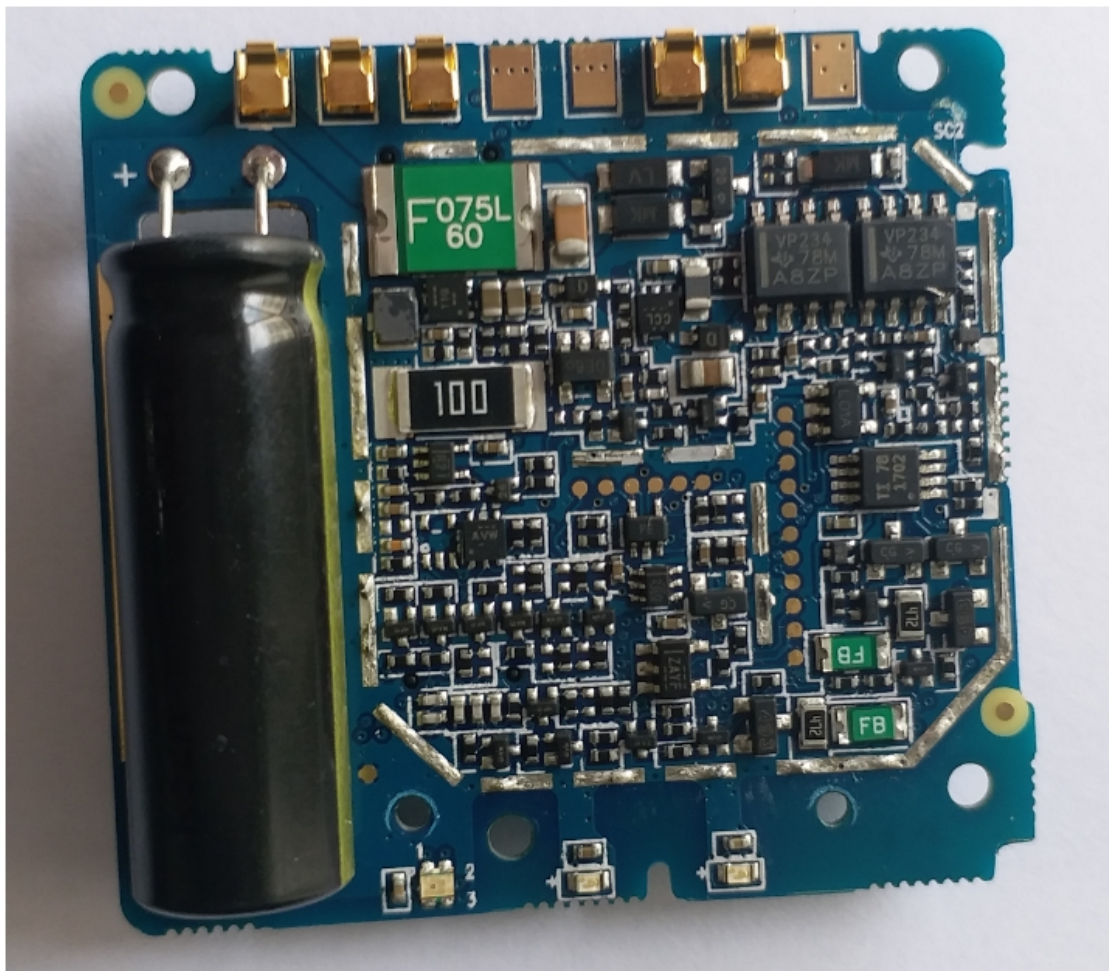
A side of OBD board without shield
