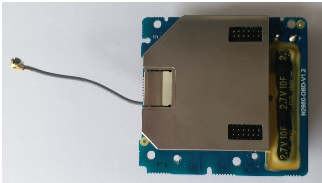
B side of OBD board with shield
