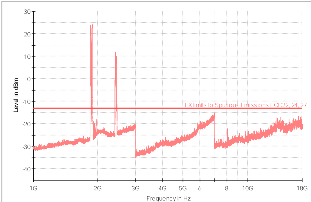
— PK+_MAXH — TX limits to Spurious Emissions FCC22, 24, 27
