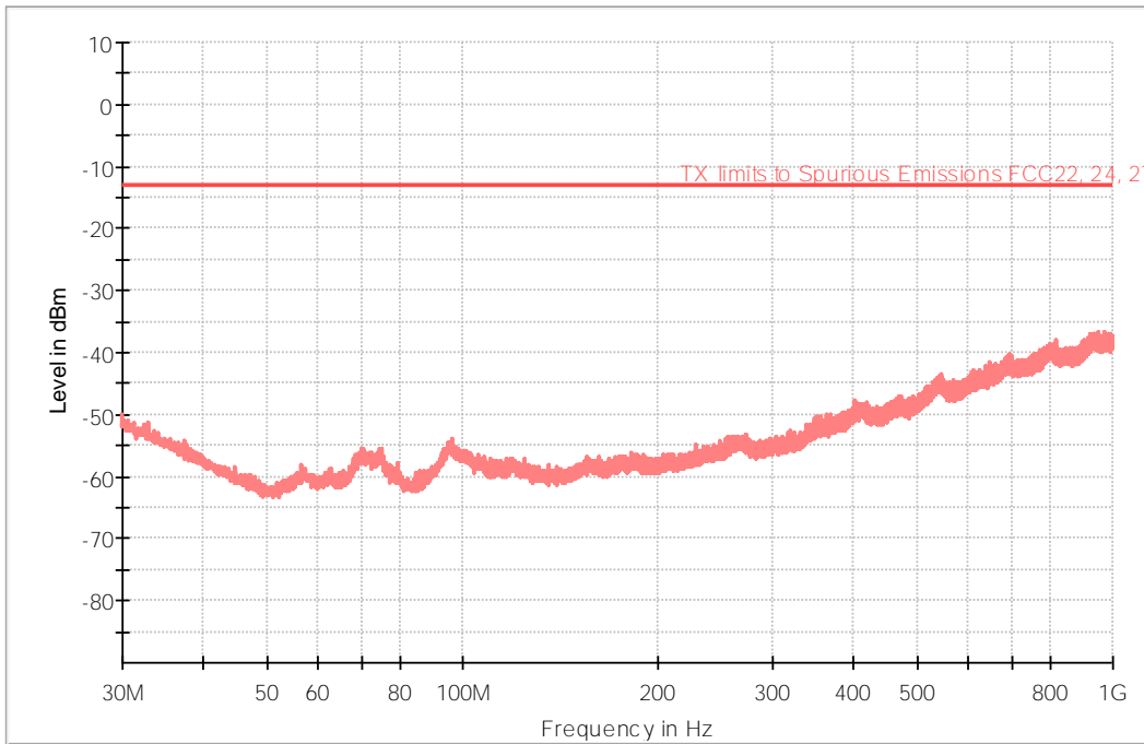
— TX limits to Spurious Emissions FCC22, 24, 27 — PK+_MAXH
