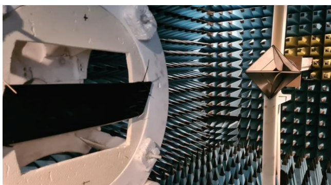
Fig. 2: Photo of DUT test set up.
