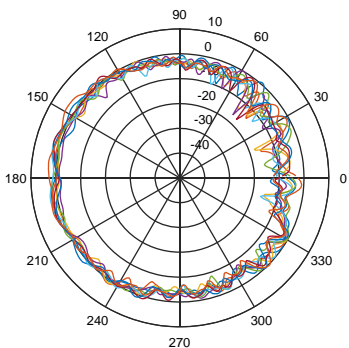
Elevation angle::140 Grad. "Horizontal+Vertical Polarisation"
