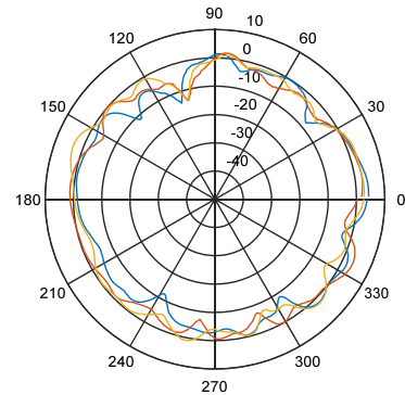
Elevation angle::90 Grad, "Horizontal+Vertical Polarisation"
