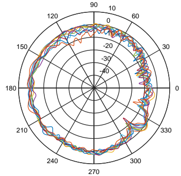
Elevation angle::160 Grad, "Horizontal+Vertical Polarisation"
