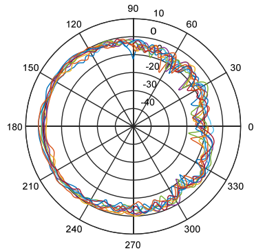
Elevation angle::90 Grad. "Horizontal+Vertical Polarisation"
