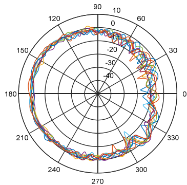
Elevation angle::120 Grad. "Horizontal+Vertical Polarisation"
