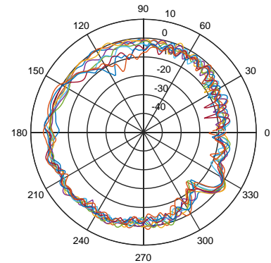
Elevation angle::180 Grad, "Horizontal+Vertical Polarisation"
