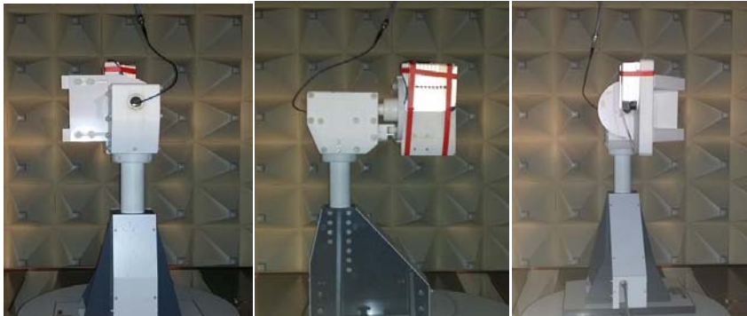
Fixed elevation angle 270°, Azimuth angle is swept from -90° to 90° The pictures show position of DUT for -90°, 0° and 90°
