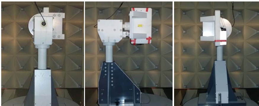
Fixed elevation angle 90°, Azimuth angle is swept from -90° to 90° The pictures show position of DUT for -90°, 0° and 90°
