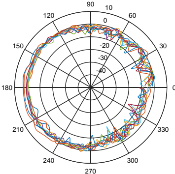
Elevation angle::270 Grad, "Horizontal+Vertical Polarisation"
