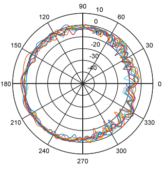
Elevation angle::140 Grad. "Horizontal+Vertical Polarisation"
