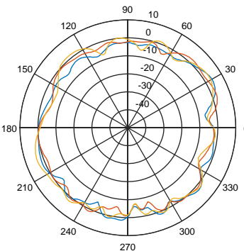
Elevation angle::200 Grad, "Horizontal+Vertical Polarisation"
