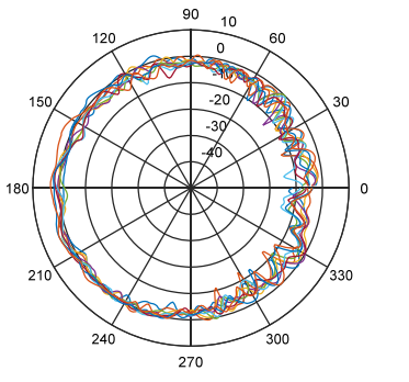
Elevation angle::140 Grad. "Horizontal+Vertical Polarisation"
