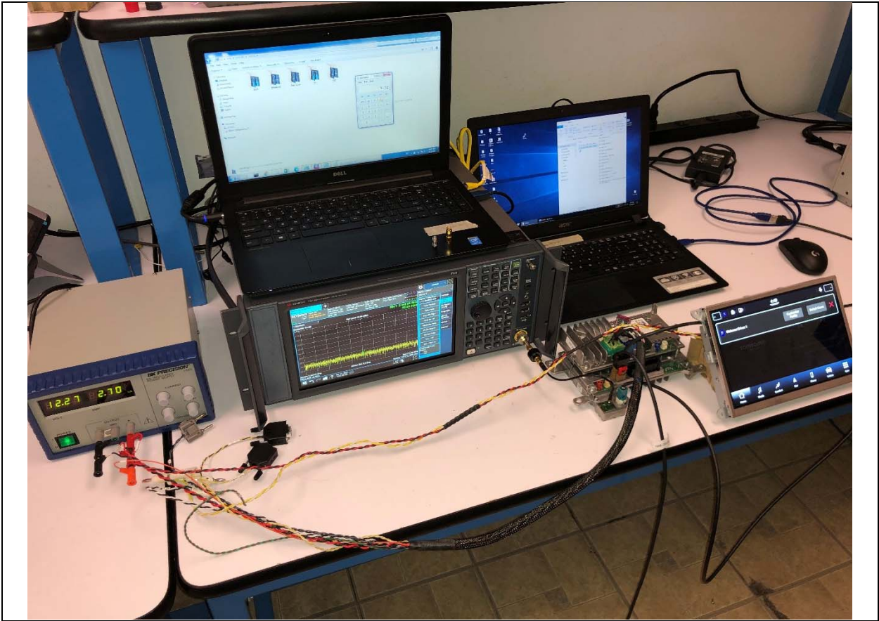
Conducted Measurement Setup
