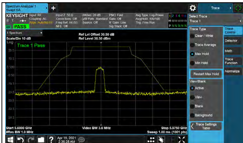
802.11a-5785MHz
