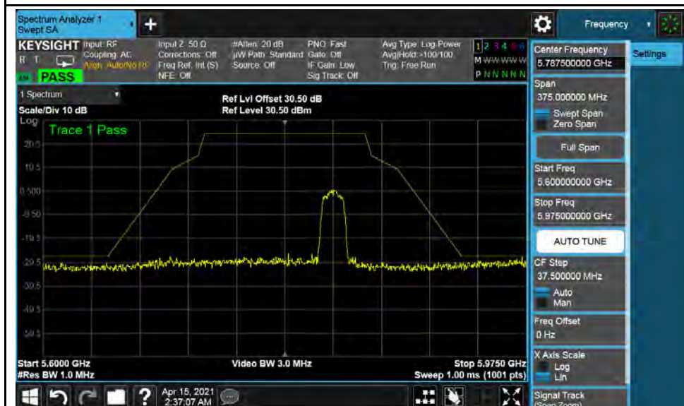
802.11a-5825MHz
