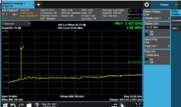
Hopping enabled 30 MHz-25 GHz
