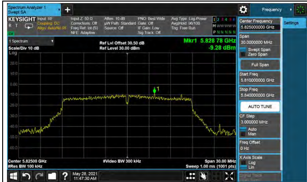
802.11ac-VHT20-5825MHz
