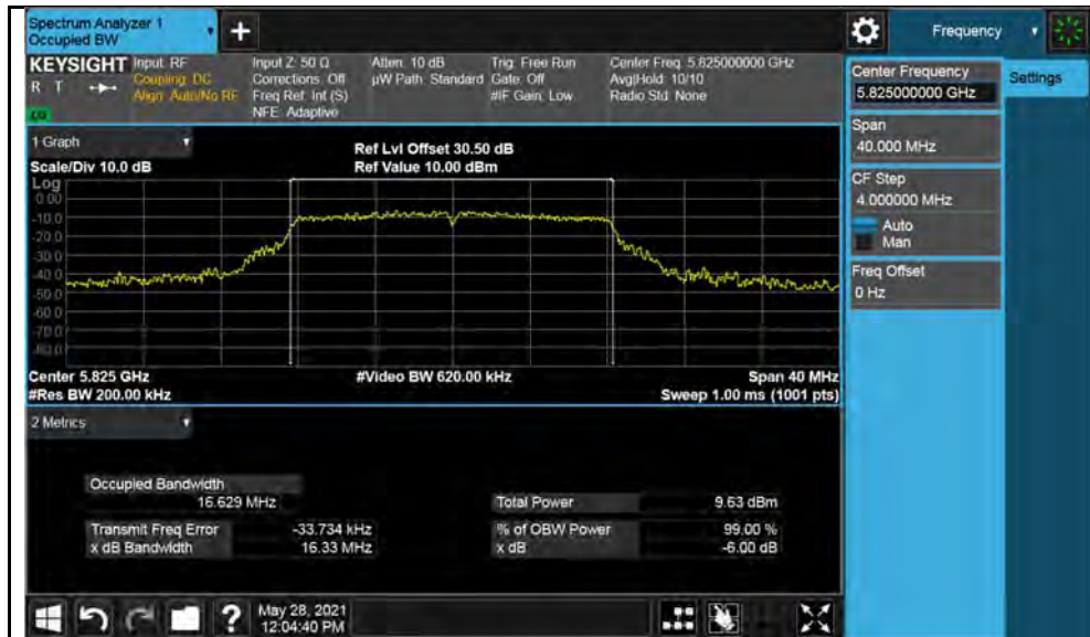
802.11a-5825MHz
