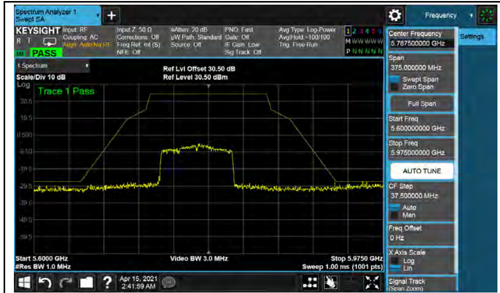
802.11n ac(VHT80)-5775MHz
