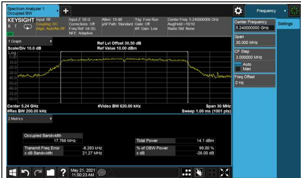
802.11ac-VHT20-5240MHz
