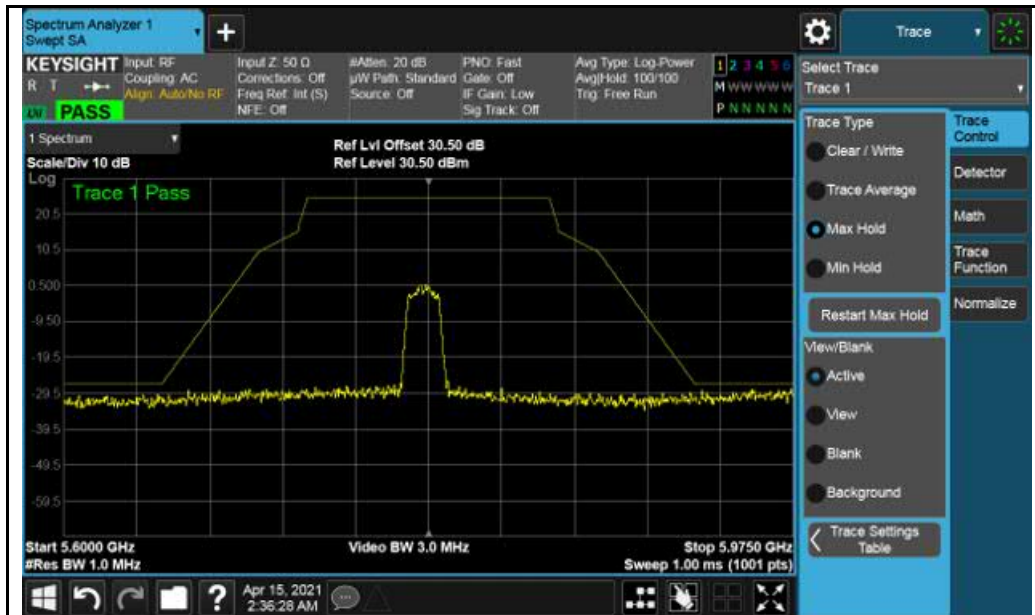
802.11a-5785MHz
