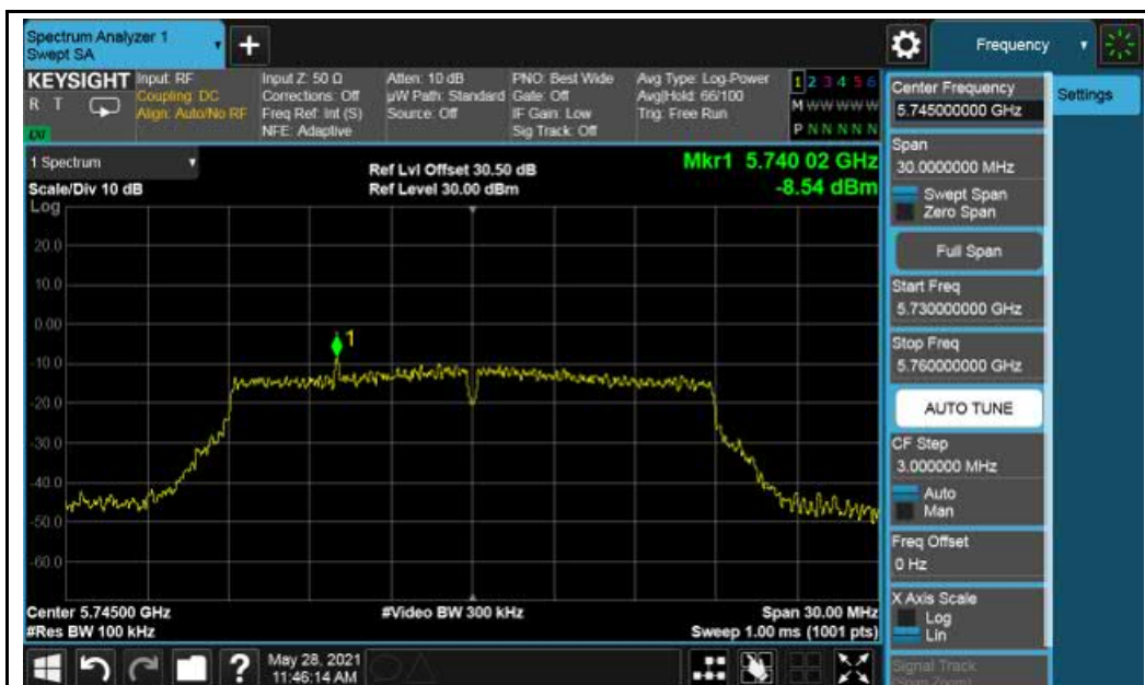
802.11ac-VHT20-5745MHz
