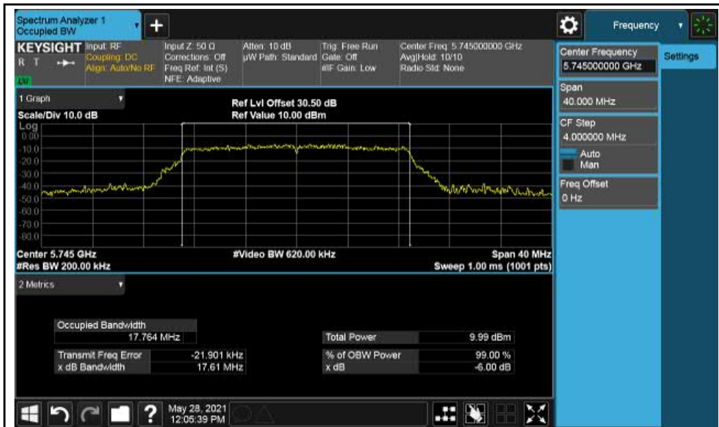
802.11ac-HT20-5745MHz
