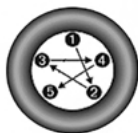
Torque Patterns
