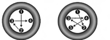
Torque Patterns
