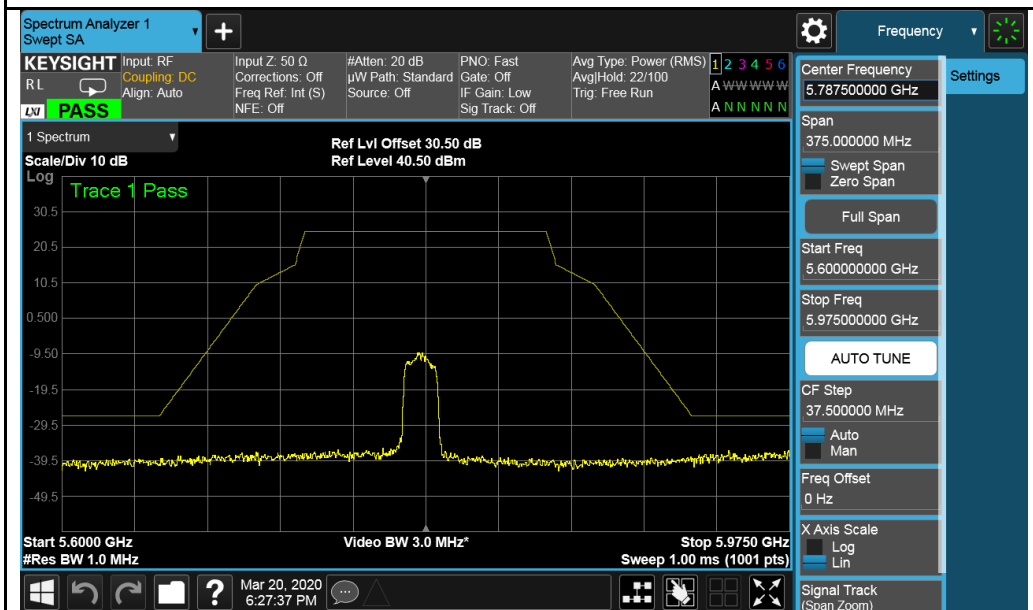
802.11a-5785MHz
