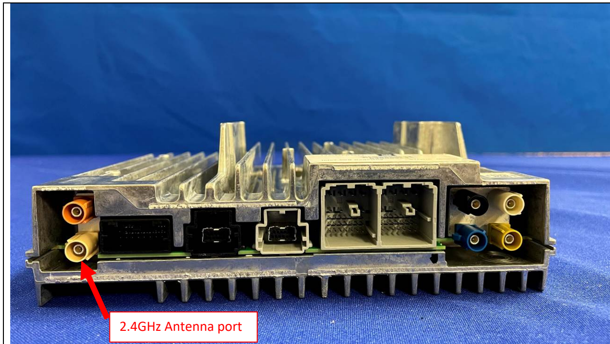
EUT I/O View
