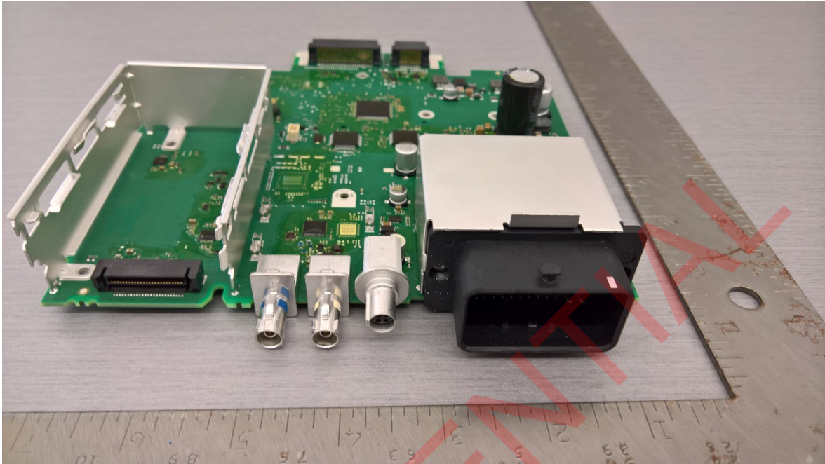
Main Board – Side View 1
