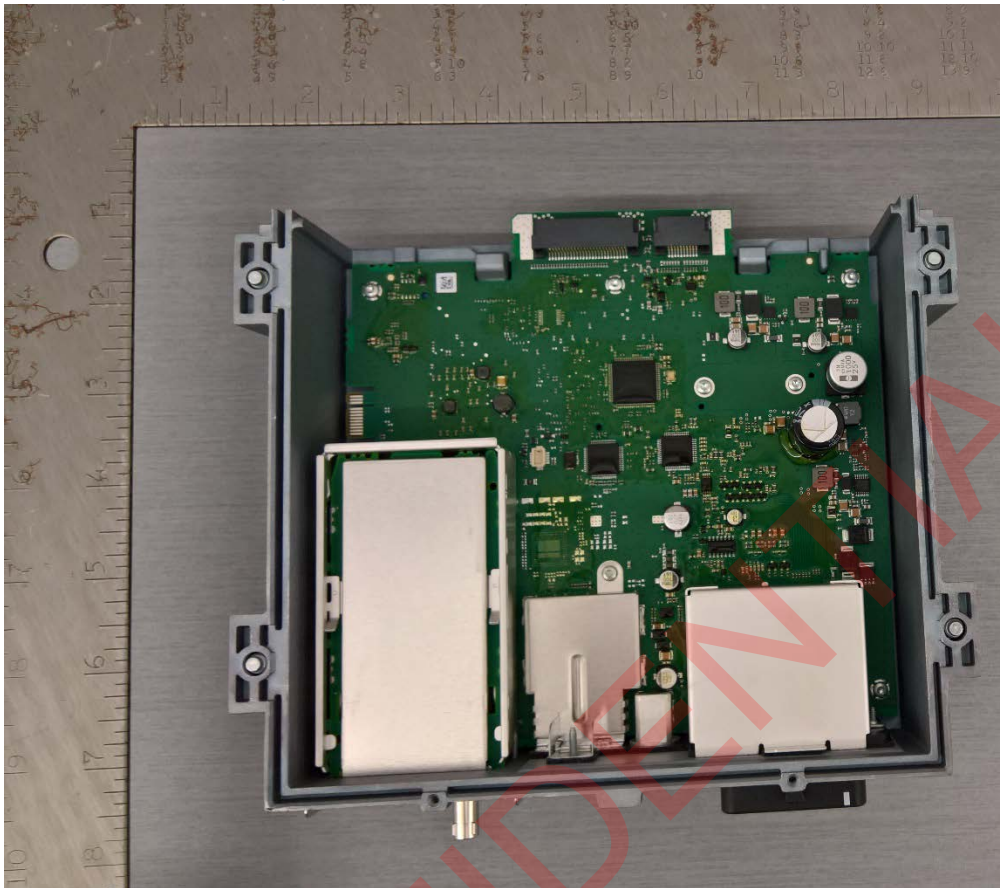
Main Board - Top – with shields and Sirius XM board
