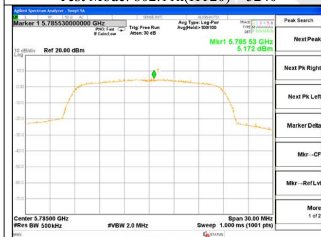
Test Mode: 802.11(HT20)---5785
