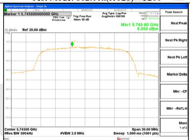
Test Mode: 802.11(HT20)---5745
