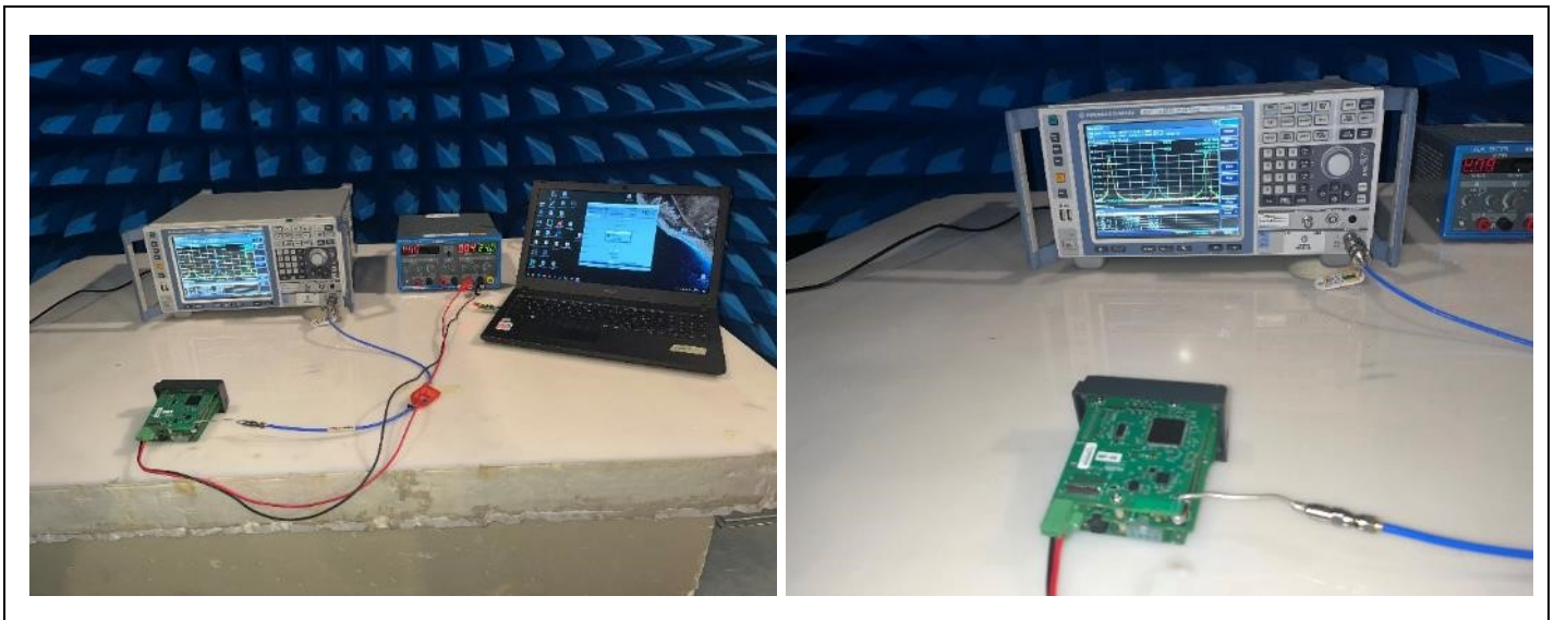
Photograph for Maximum Conducted Output Power
