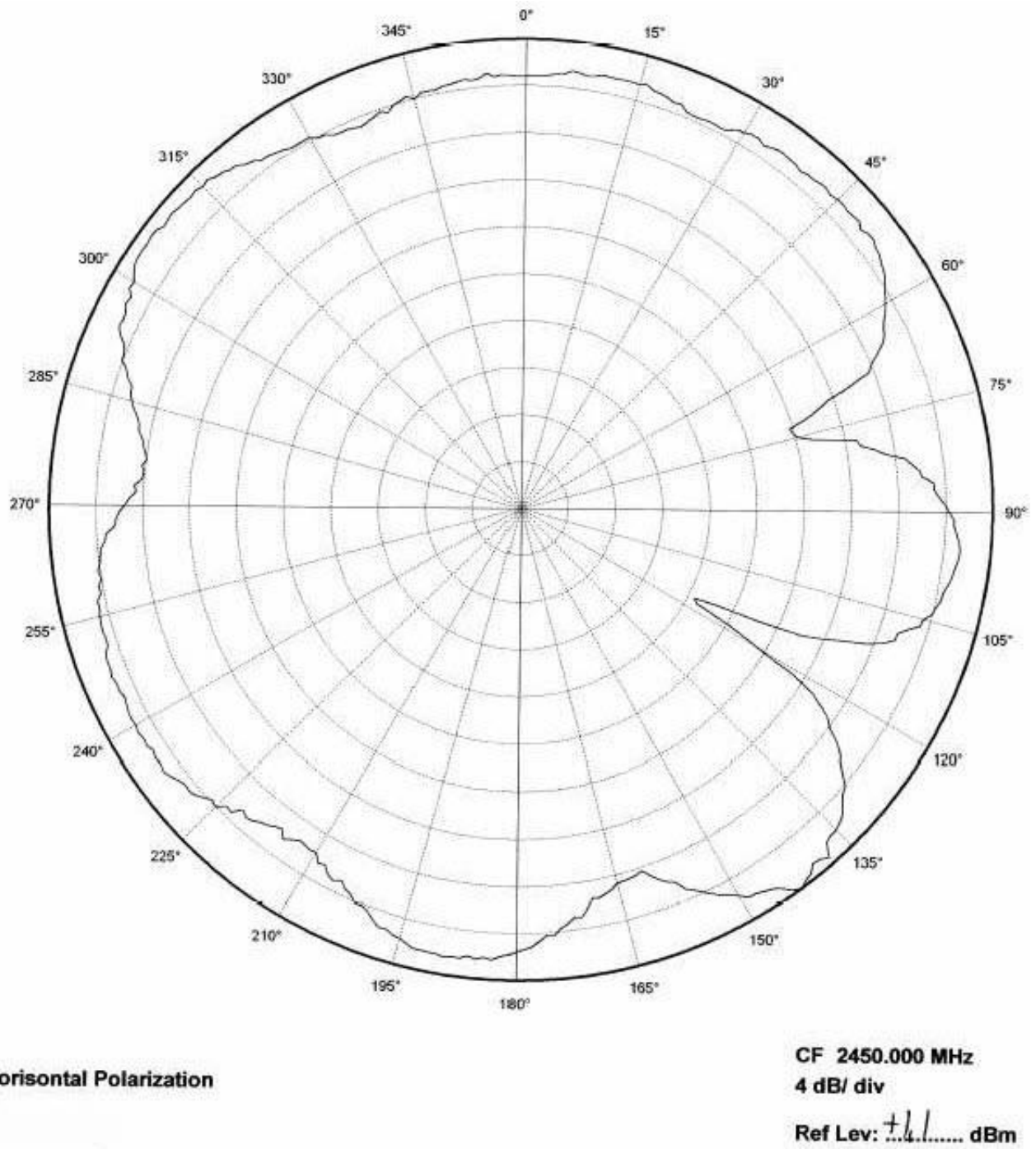
Figure 4. XY Plane Horizontal Polarization
