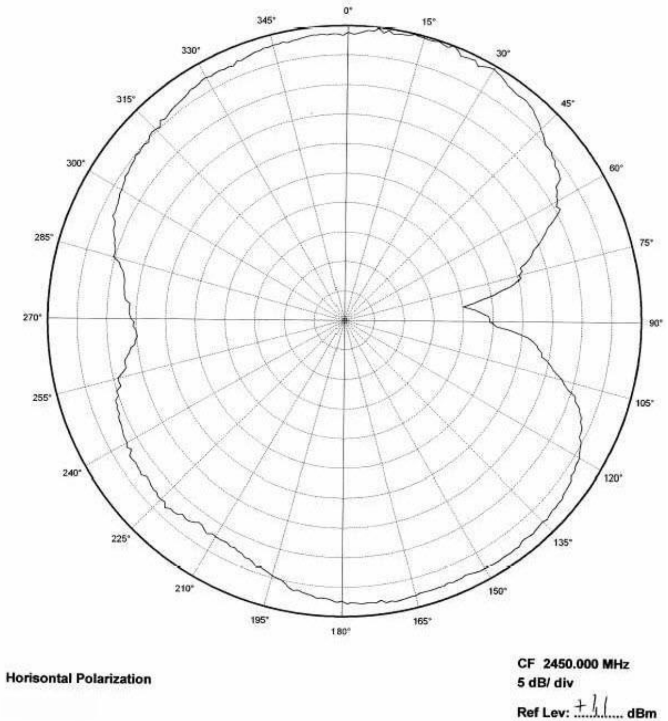
Figure 8. YZ Plane Horizontal Polarization
