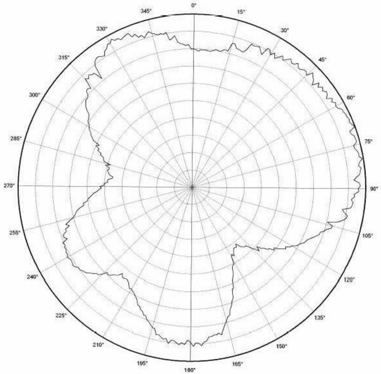
Figure 5. XZ Plane Vertical Polarization
