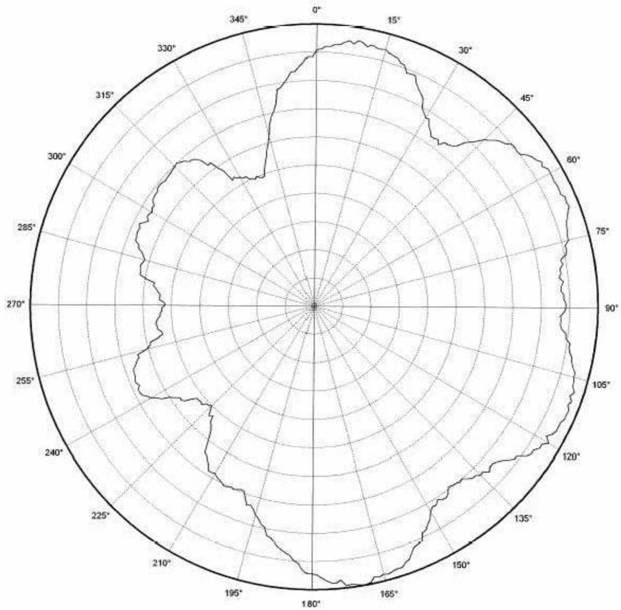
Figure 6. XZ Plane Horizontal Polarization
