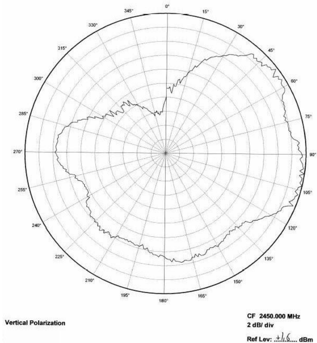
Figure 7. YZ Plane Vertical Polarization
