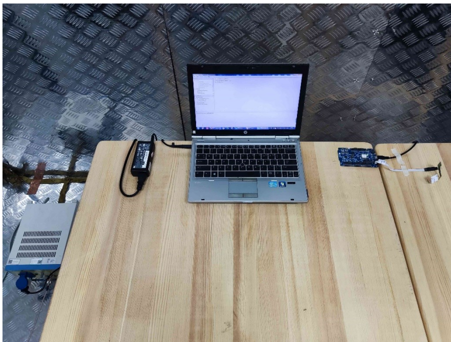
Conducted Emission test view_AC
