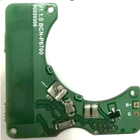
EUT bottom side view_RADMEDIA-BLE-T22
