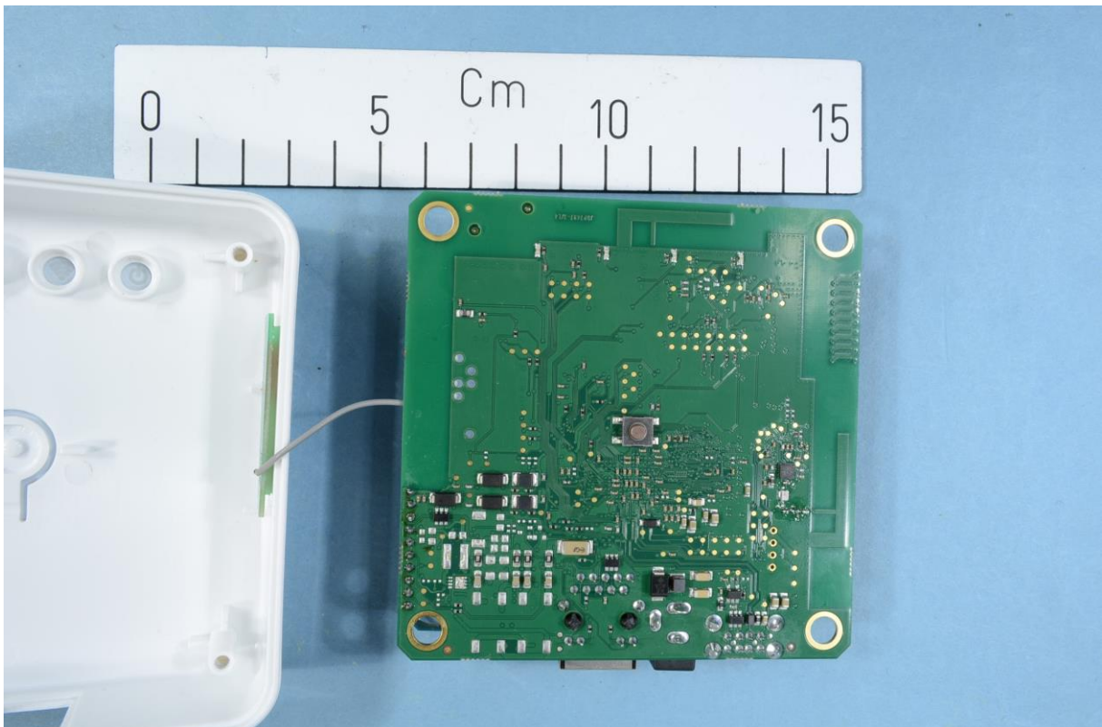
SquidLink – Rear view of PCB
