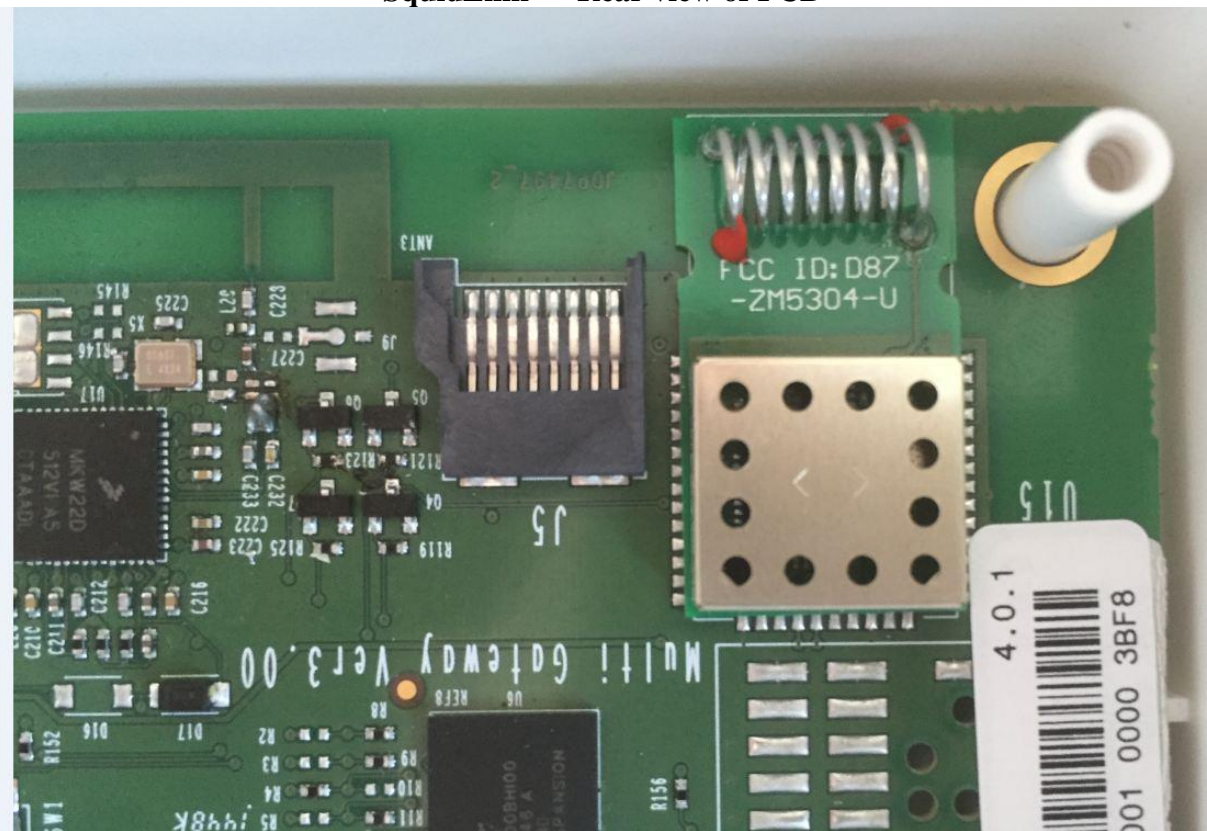
SquidLink – view of ZWave module
