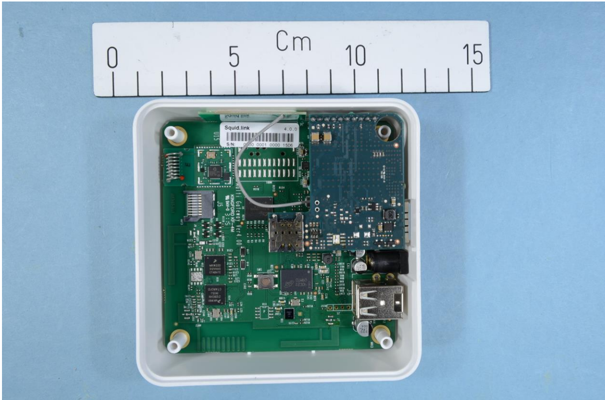
SquidLink – Front view of PCB
