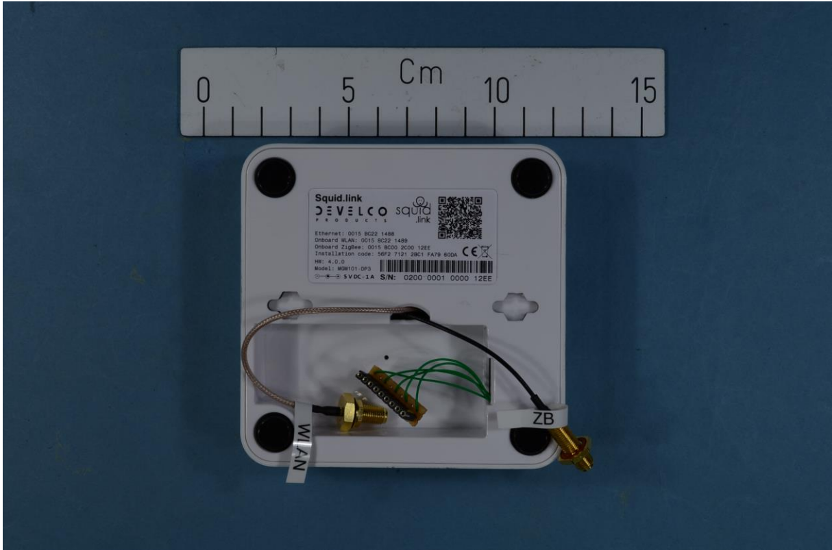
SquidLink – for conducted measurements
