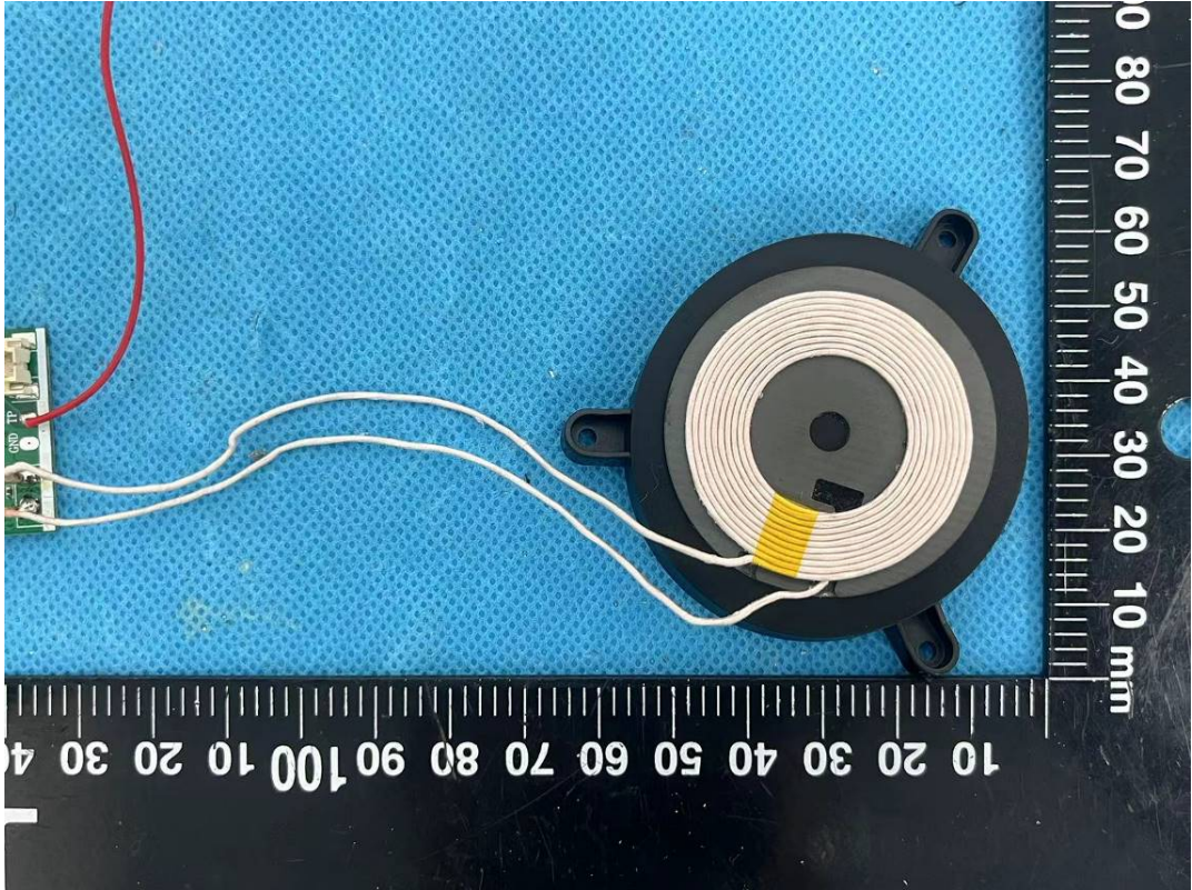
Coil Antenna
