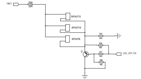
Lamp circuit
