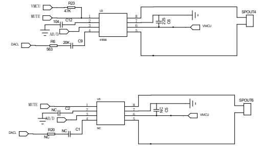
Power amplifier circuit
