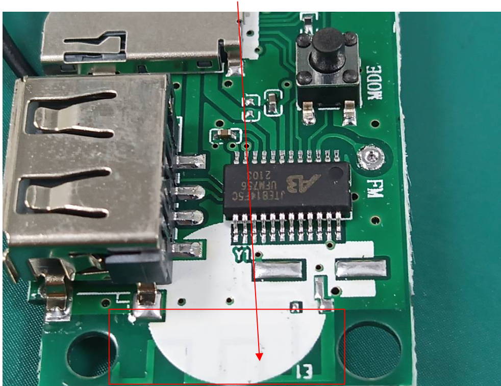
Bluetooth Antenna
